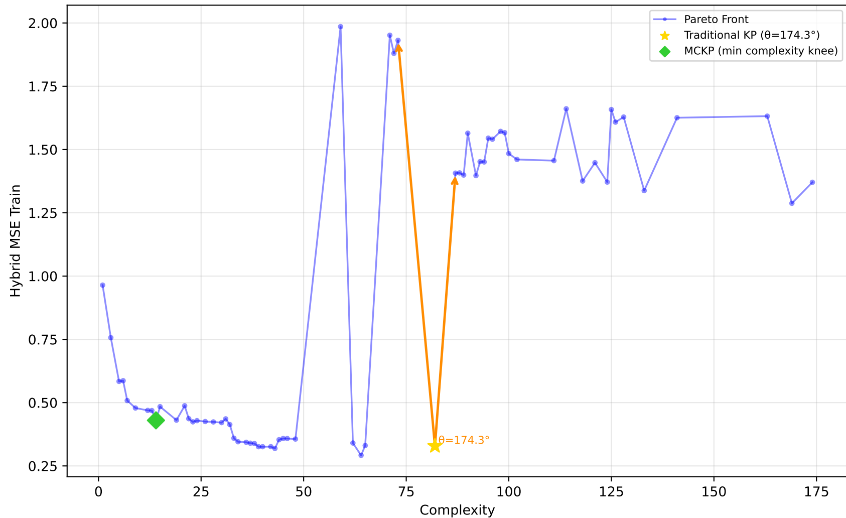
192_vineyard - Run 10 - SVP - Hybrid MSE Train \lambda_1=0.70, \lambda_2=0.70, \lambda_3=0.90 | Difficulty: 0.17 | Method: mckp
