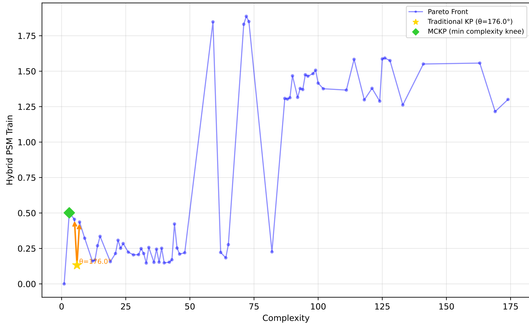
192_vineyard - Run 10 - SVP - Hybrid PSM Train \lambda_1=0.70, \lambda_2=0.70, \lambda_3=0.90 | Difficulty: 0.17 | Method: mckp
