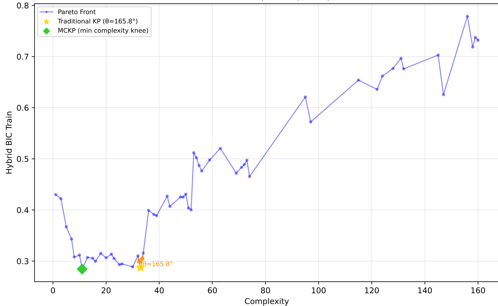
192_vineyard - Run 11 - MVP - Hybrid BIC Train \lambda_1=0.40, \bar{\lambda}_2=0.00, \lambda_3=1.00 | Difficulty: 1.00 | Method: hmr
