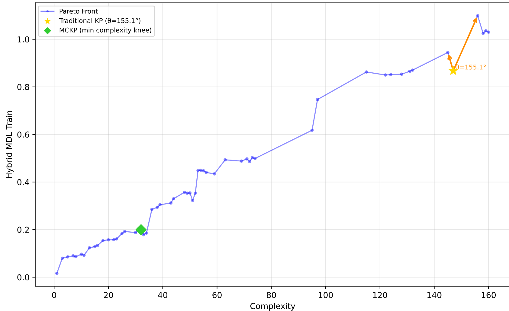
192_vineyard - Run 11 - MVP - Hybrid MDL Train \lambda_1=0.40, \bar{\lambda}_2=0.00, \lambda_3=1.00 | Difficulty: 1.00 | Method: hmr
