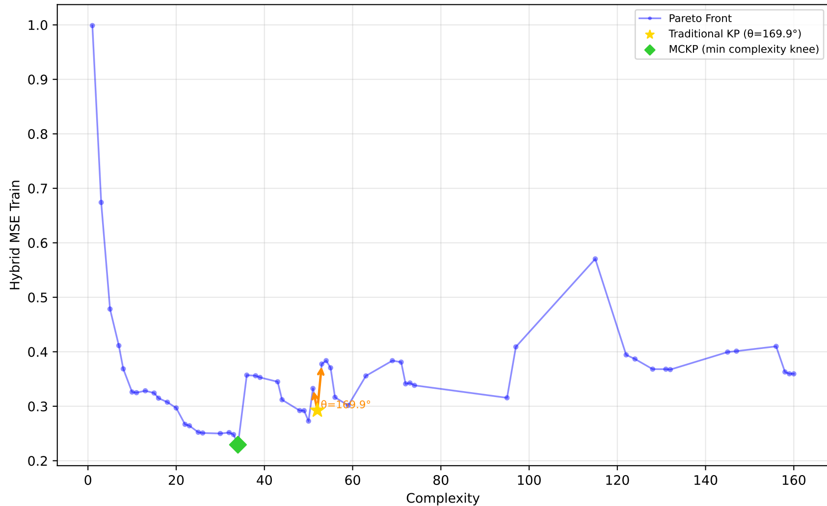
192_vineyard - Run 11 - SVP - Hybrid MSE Train \lambda_1=0.00, \lambda_2=1.00, \lambda_3=1.00 | Difficulty: 1.00 | Method: hmr
