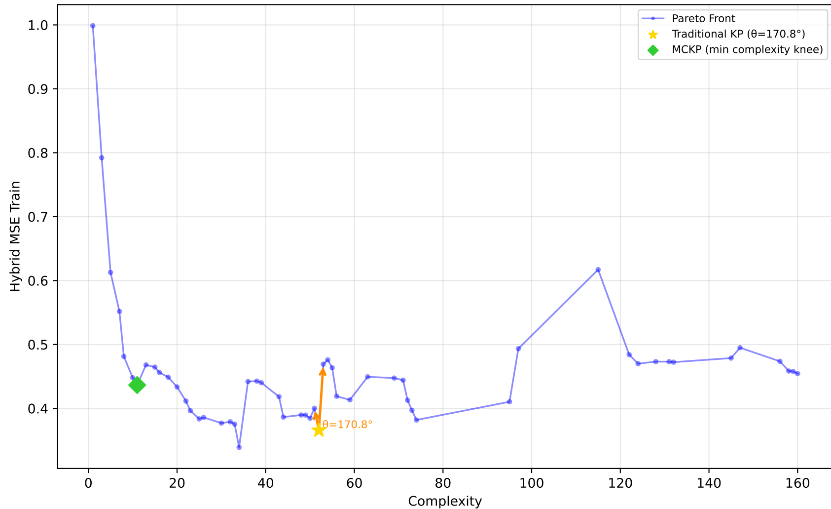
192_vineyard - Run 11 - SVP - Hybrid MSE Train \lambda_1=0.70, \lambda_2=0.70, \lambda_3=0.90 | Difficulty: 1.00 | Method: hmr
