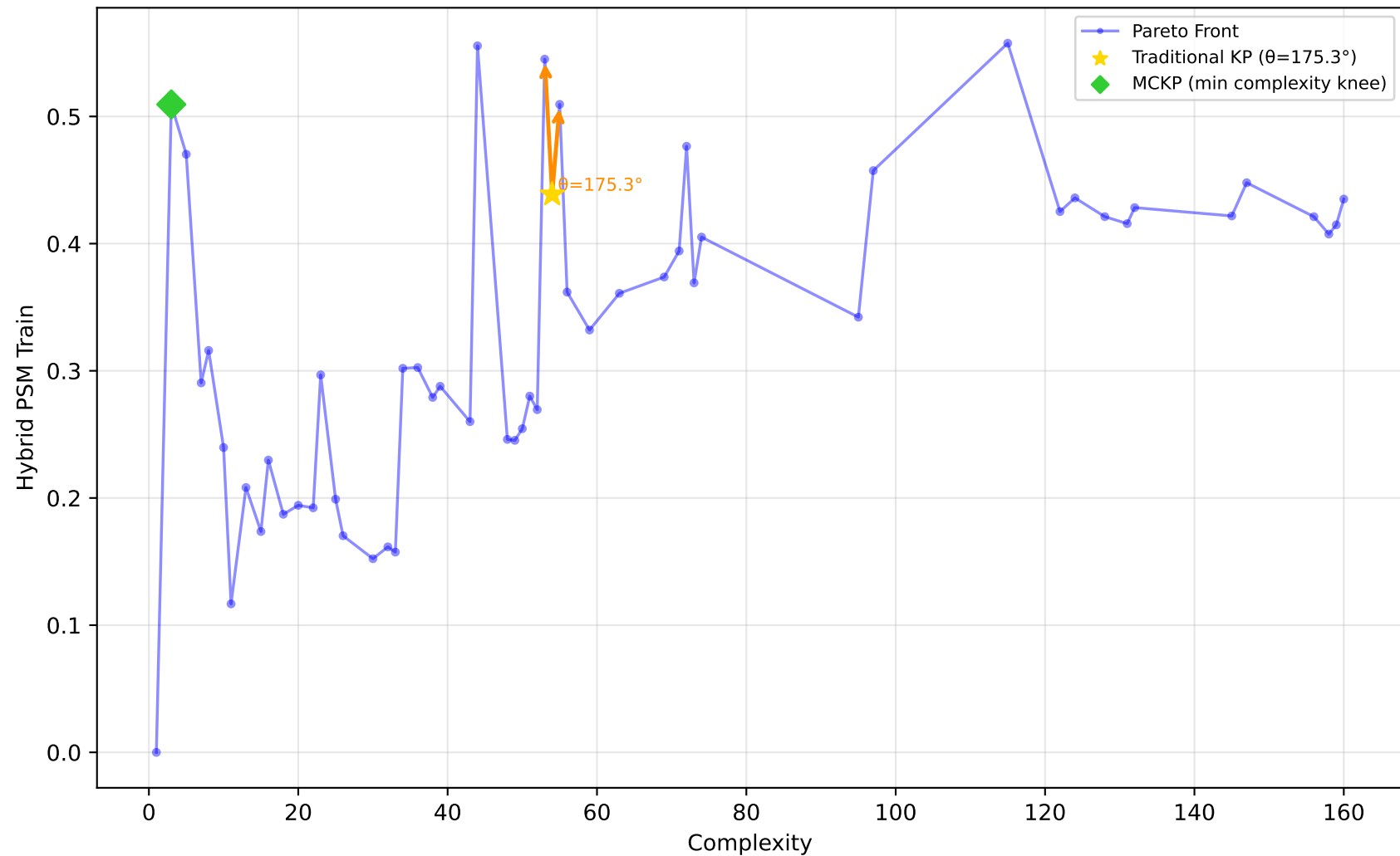
192_vineyard - Run 11 - SVP - Hybrid PSM Train \lambda_1=0.70, \bar{\lambda}_2=0.70, \lambda_3=0.90 | Difficulty: 1.00 | Method: hmr
