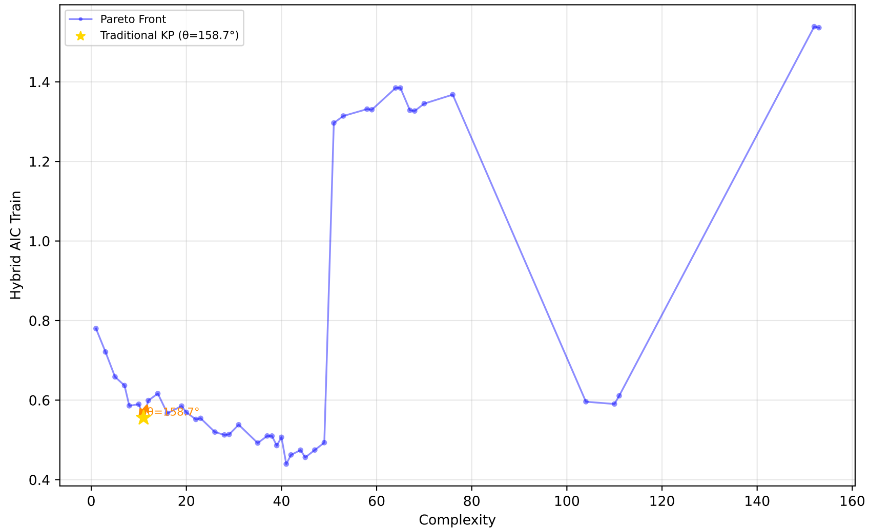
192_vineyard - Run 12 - MVP - Hybrid AIC Train \lambda_1=0.40, \lambda_2=0.00, \lambda_3=1.00 | Difficulty: 0.20 | Method: mckp
