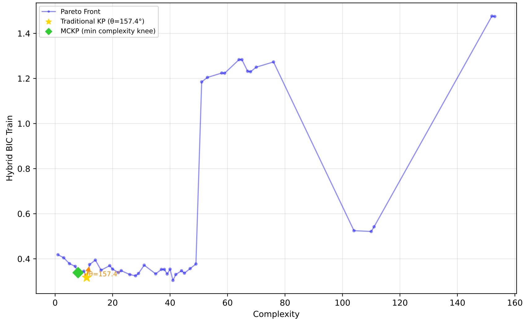
192_vineyard - Run 12 - MVP - Hybrid BIC Train \lambda_1=0.40, \lambda_2=0.00, \lambda_3=1.00 | Difficulty: 0.20 | Method: mckp
