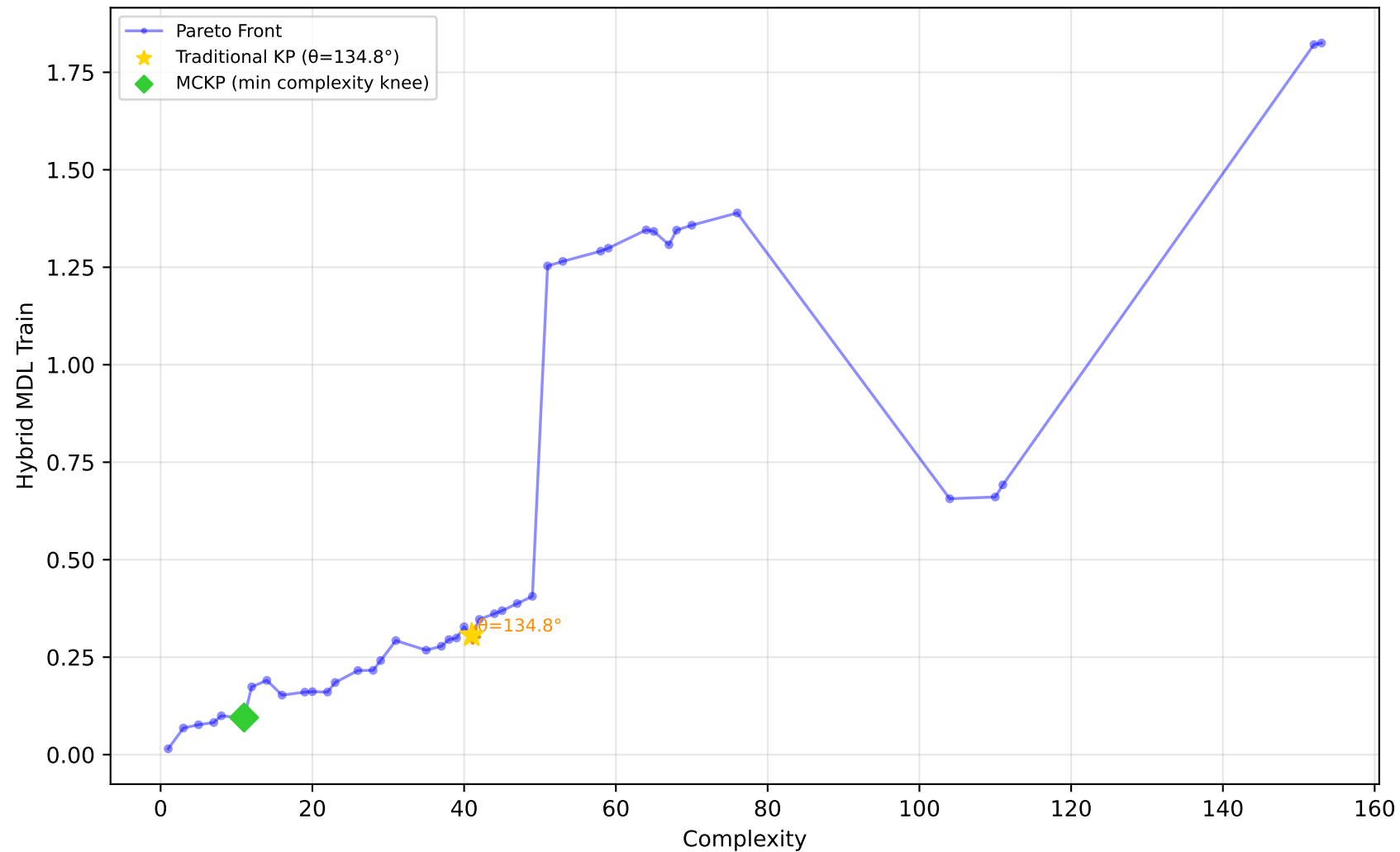
192_vineyard - Run 12 - MVP - Hybrid MDL Train \lambda_1=0.40, \bar{\lambda}_2=0.00, \lambda_3=1.00 | Difficulty: 0.20 | Method: mckp
