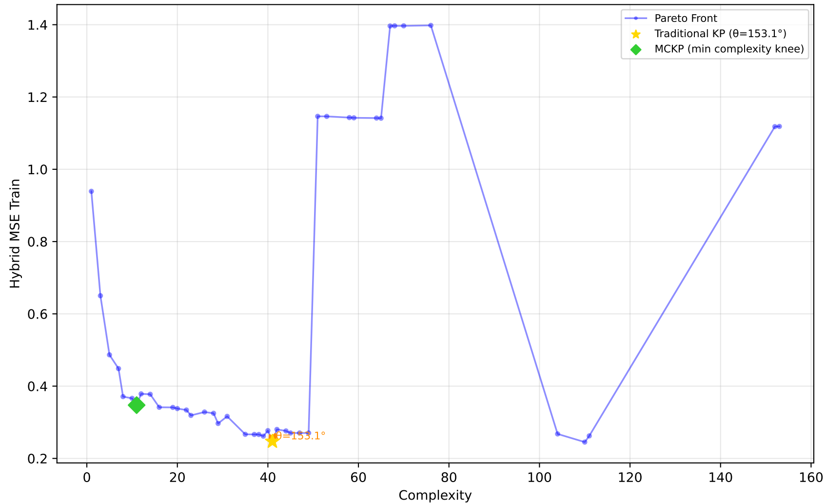
192_vineyard - Run 12 - MVP - Hybrid MSE Train \lambda_1=0.00, \bar{\lambda}_2=0.30, \lambda_3=1.00 | Difficulty: 0.20 | Method: mckp
