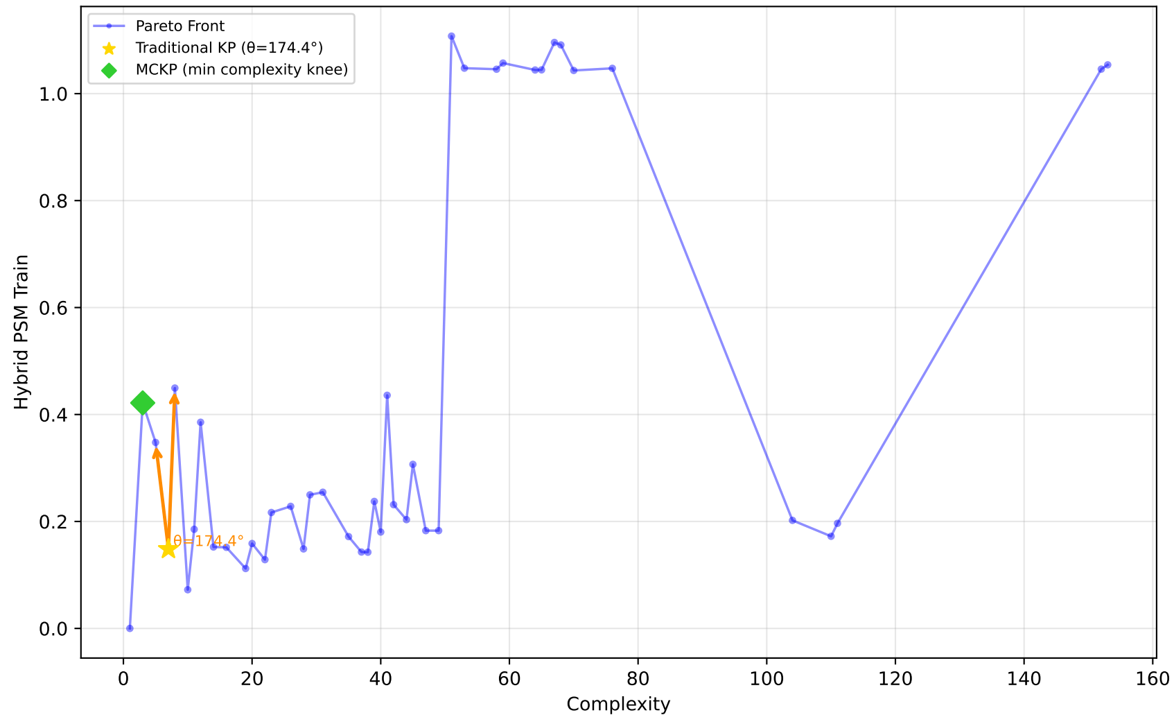
192_vineyard - Run 12 - MVP - Hybrid PSM Train \lambda_1=0.40, \bar{\lambda}_2=0.00, \lambda_3=1.00 | Difficulty: 0.20 | Method: mckp
