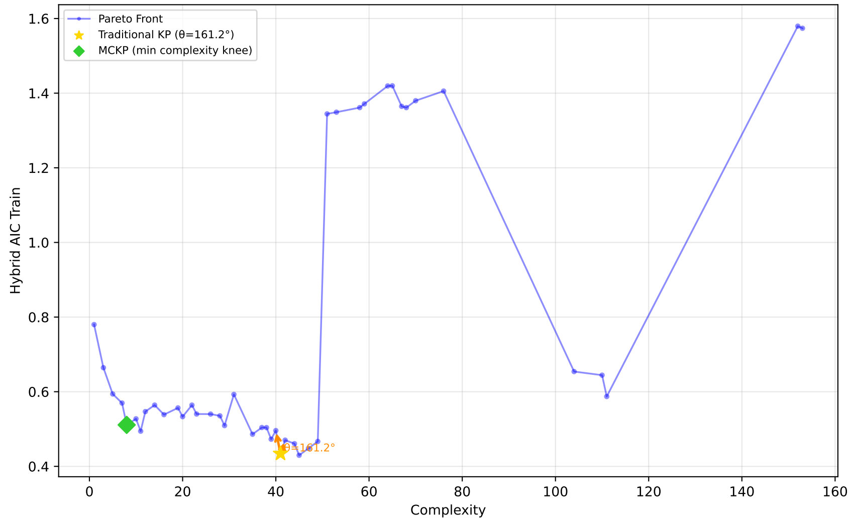
192_vineyard - Run 12 - SVP - Hybrid AIC Train \lambda_1=0.00, \lambda_2=1.00, \lambda_3=1.00 | Difficulty: 0.20 | Method: mckp
