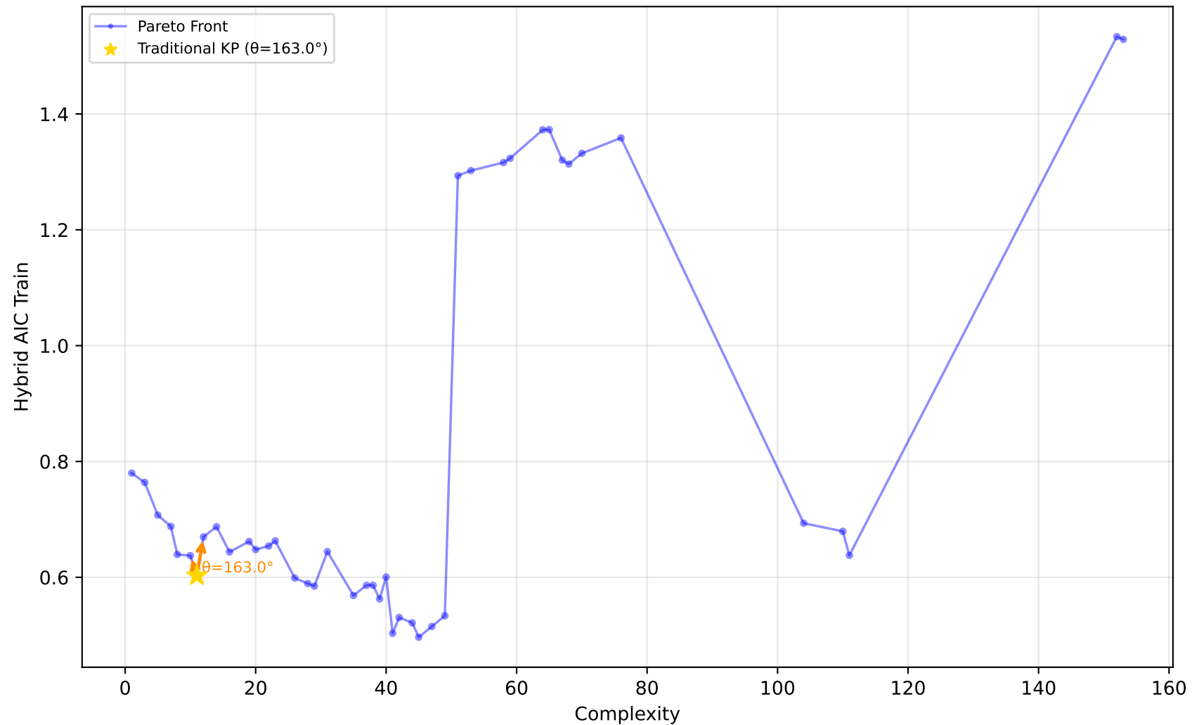
192_vineyard - Run 12 - SVP - Hybrid AIC Train \lambda_1=0.70, \lambda_2=0.70, \lambda_3=0.90 | Difficulty: 0.20 | Method: mckp
