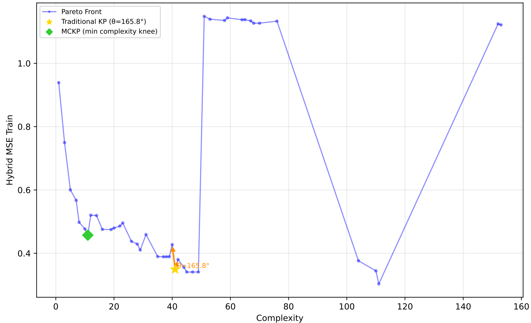
192_vineyard - Run 12 - SVP - Hybrid MSE Train \lambda_1=0.70, \lambda_2=0.70, \lambda_3=0.90 | Difficulty: 0.20 | Method: mckp
