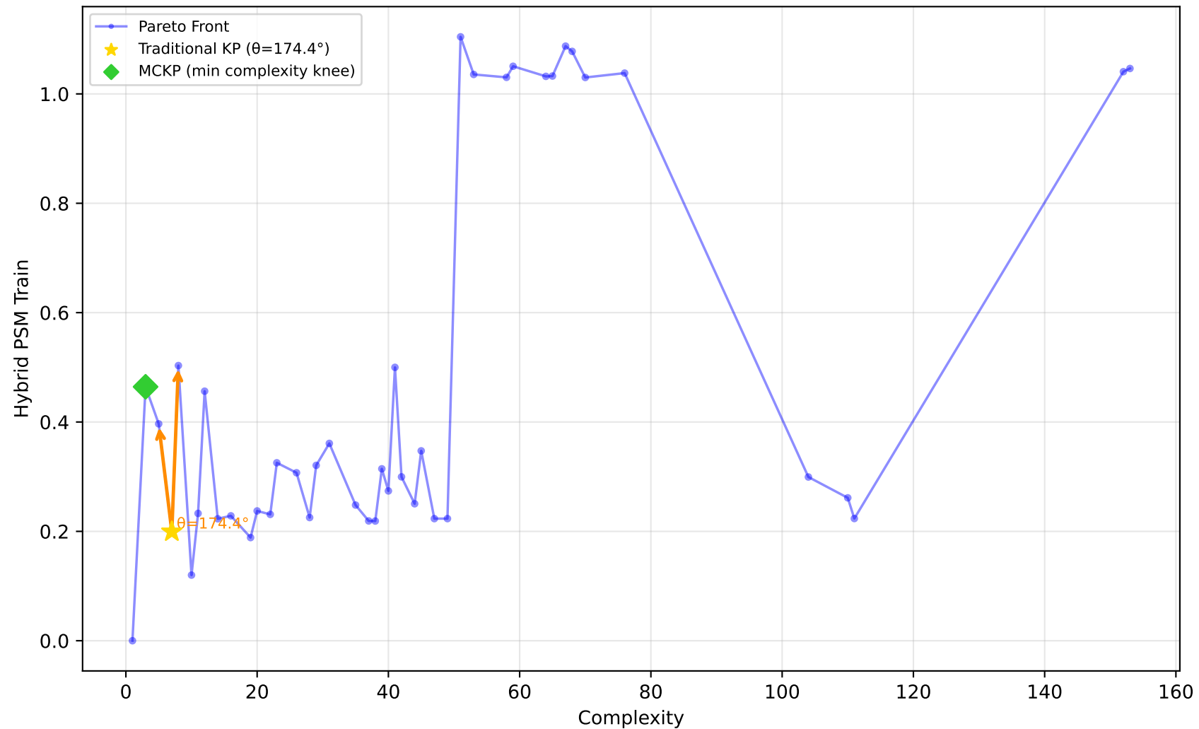
192_vineyard - Run 12 - SVP - Hybrid PSM Train \lambda_1=0.70, \lambda_2=0.70, \lambda_3=0.90 | Difficulty: 0.20 | Method: mckp
