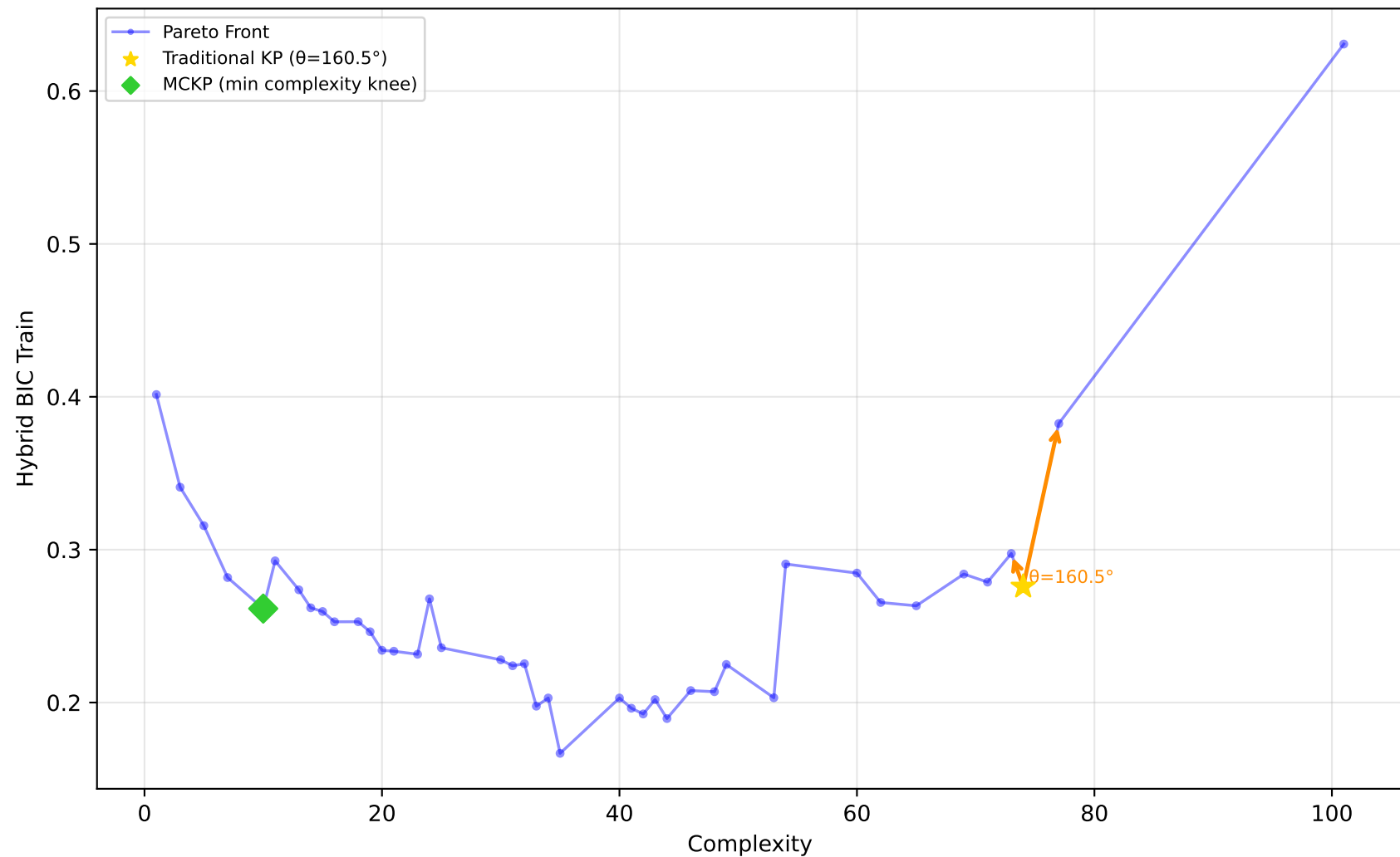
192_vineyard - Run 13 - MVP - Hybrid BIC Train \lambda_1=0.00, \bar{\lambda}_2=0.30, \lambda_3=1.00 | Difficulty: 0.67 | Method: hmr
