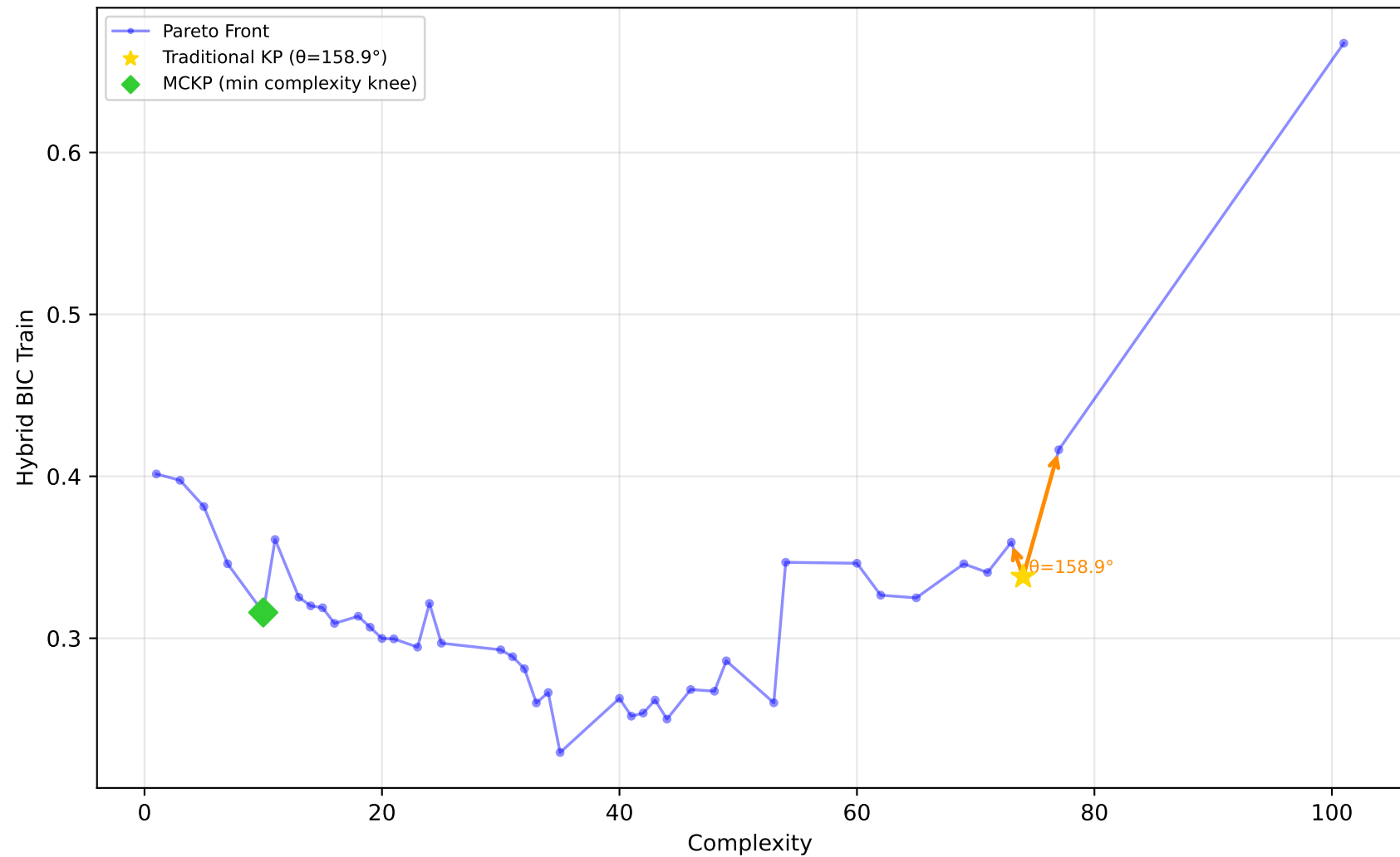
192_vineyard - Run 13 - MVP - Hybrid BIC Train \lambda_1=0.40, \bar{\lambda}_2=0.00, \lambda_3=1.00 | Difficulty: 0.67 | Method: hmr
