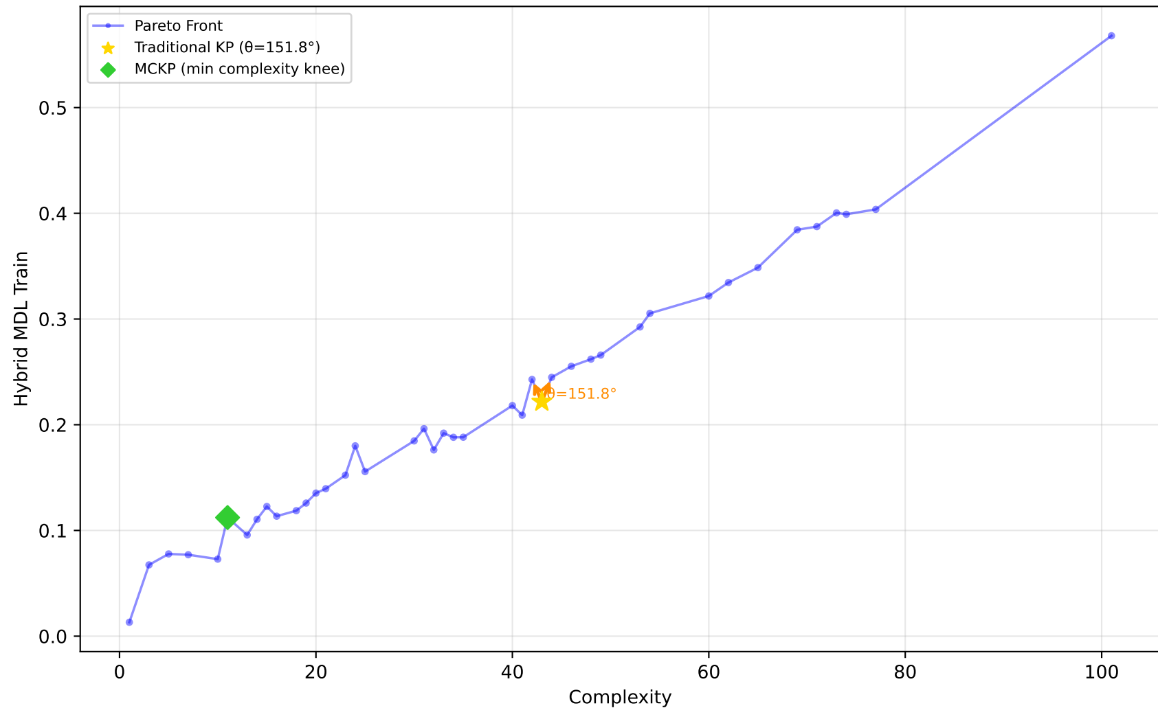
192_vineyard - Run 13 - MVP - Hybrid MDL Train \lambda_1=0.40, \lambda_2=0.00, \lambda_3=1.00 | Difficulty: 0.67 | Method: hmr
