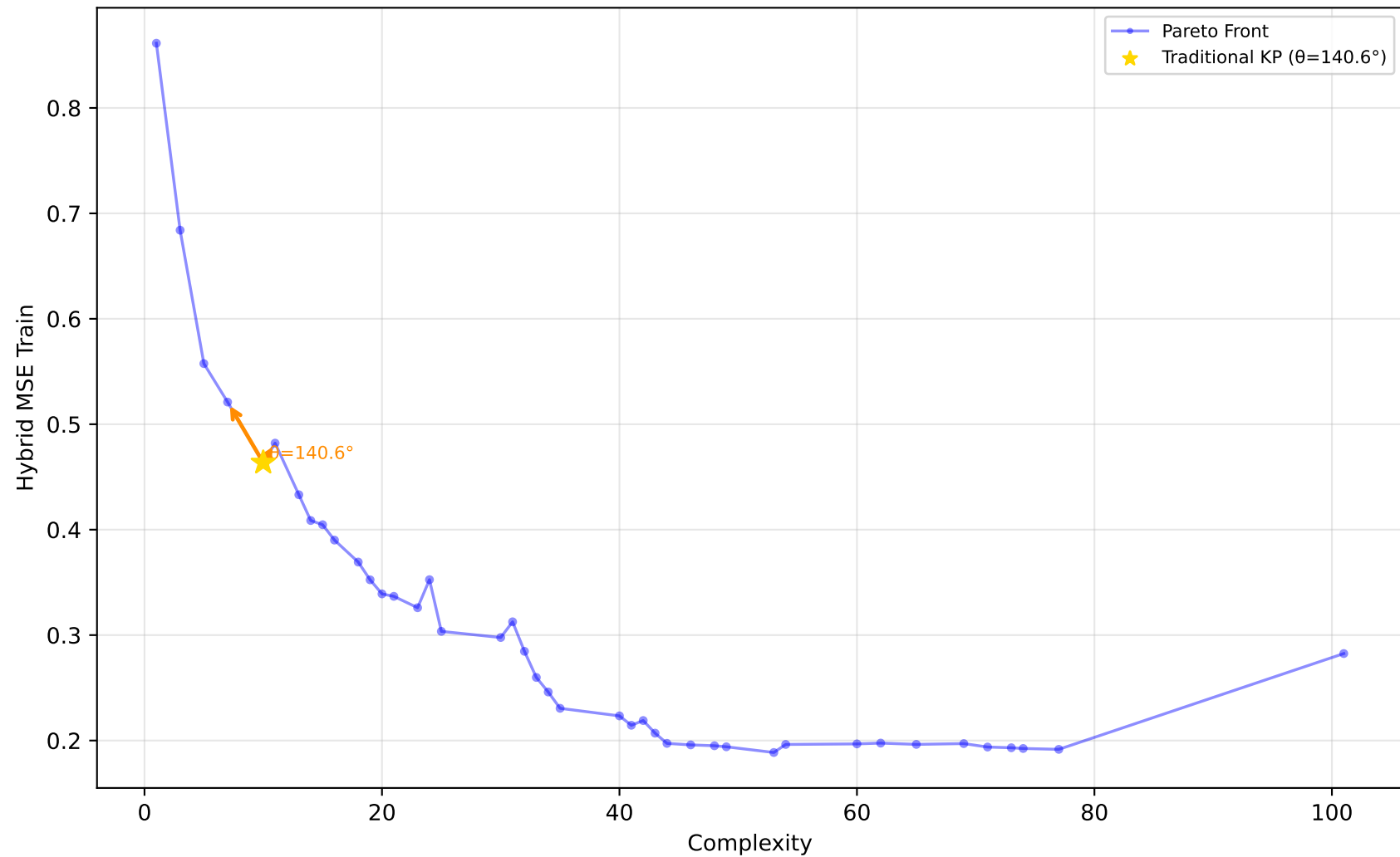
192_vineyard - Run 13 - MVP - Hybrid MSE Train \lambda_1=0.40, \lambda_2=0.00, \lambda_3=1.00 | Difficulty: 0.67 | Method: hmr
