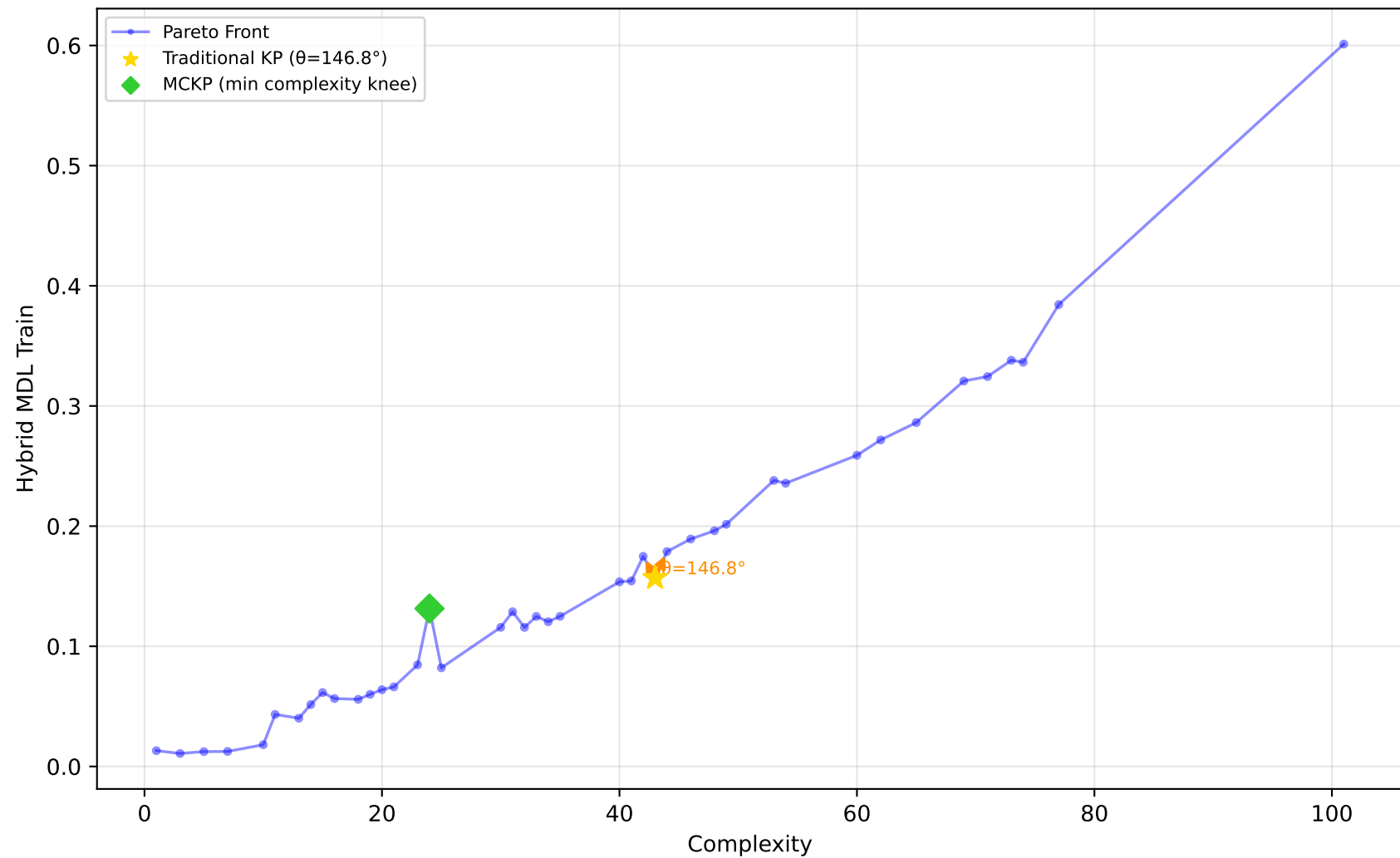
192_vineyard - Run 13 - SVP - Hybrid MDL Train \lambda_1=0.00, \bar{\lambda}_2=1.00, \lambda_3=1.00 | Difficulty: 0.67 | Method: hmr
