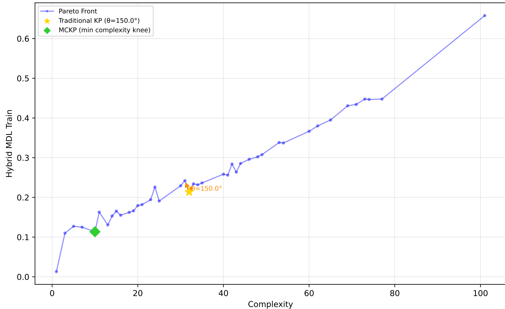
192_vineyard - Run 13 - SVP - Hybrid MDL Train \lambda_1=0.70, \bar{\lambda}_2=0.70, \lambda_3=0.90 | Difficulty: 0.67 | Method: hmr
