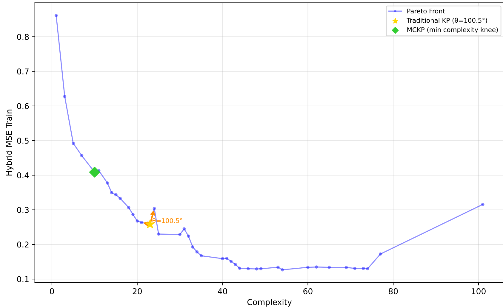
192_vineyard - Run 13 - SVP - Hybrid MSE Train \lambda_1=0.00, \lambda_2=1.00, \lambda_3=1.00 | Difficulty: 0.67 | Method: hmr
