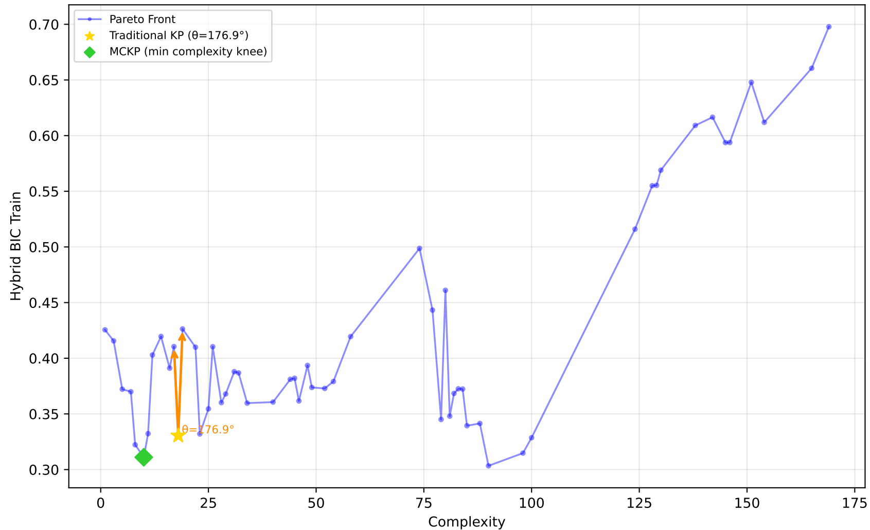
192_vineyard - Run 14 - MVP - Hybrid BIC Train \lambda_1=0.40, \bar{\lambda}_2=0.00, \lambda_3=1.00 | Difficulty: 0.72 | Method: hmr
