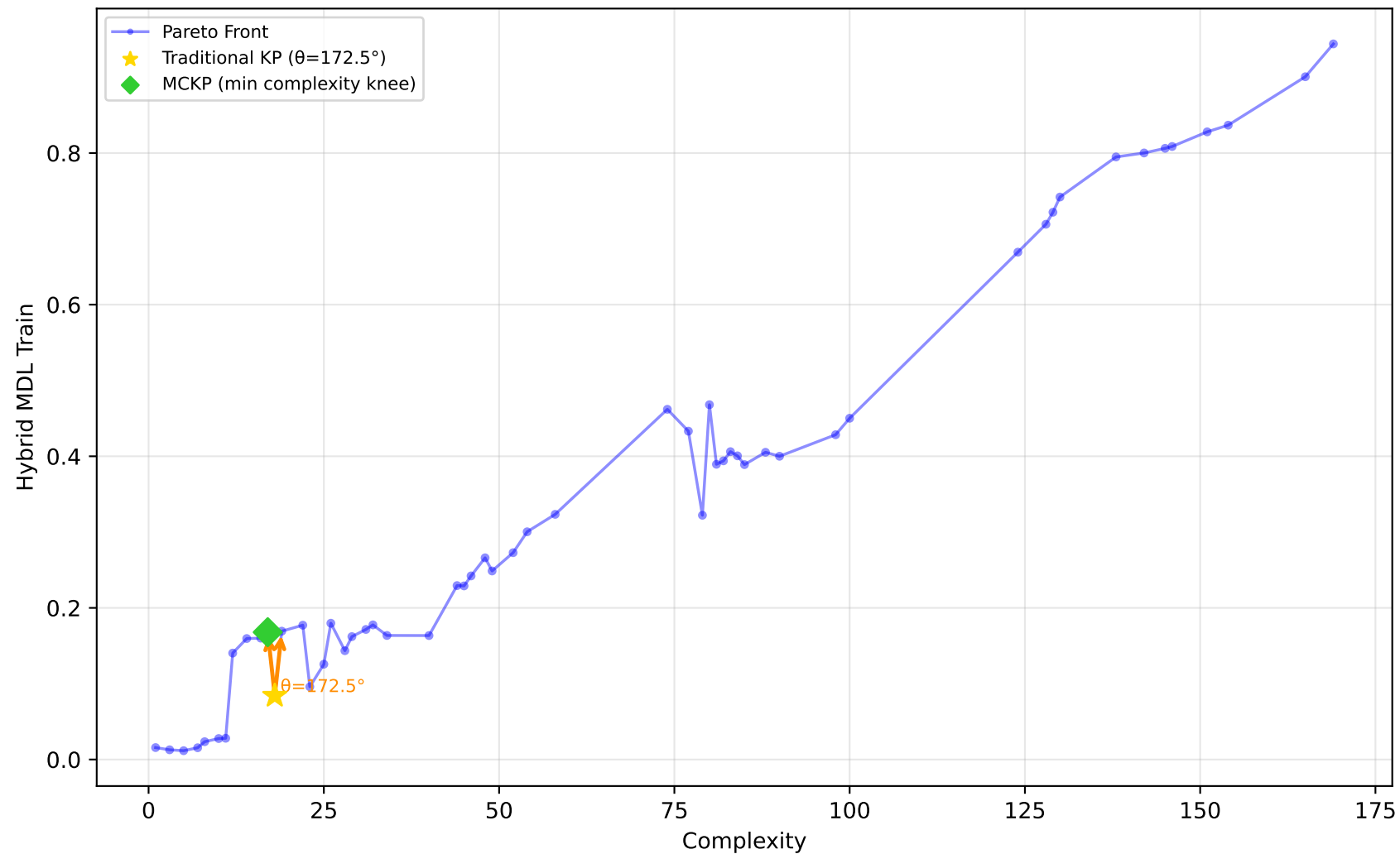
192_vineyard - Run 14 - MVP - Hybrid MDL Train \lambda_1=0.00, \bar{\lambda}_2=0.30, \lambda_3=1.00 | Difficulty: 0.72 | Method: hmr
