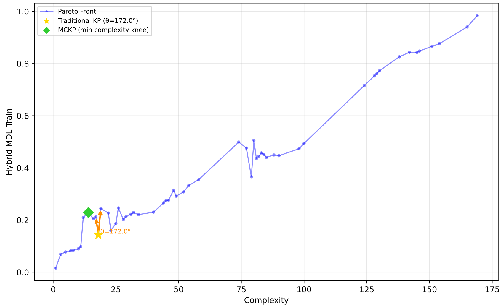
192_vineyard - Run 14 - MVP - Hybrid MDL Train \lambda_1=0.40, \bar{\lambda}_2=0.00, \lambda_3=1.00 | Difficulty: 0.72 | Method: hmr
