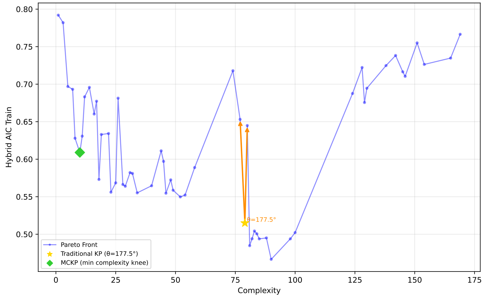
192_vineyard - Run 14 - SVP - Hybrid AIC Train \lambda_1=0.70, \bar{\lambda}_2=0.70, \lambda_3=0.90 | Difficulty: 0.72 | Method: hmr
