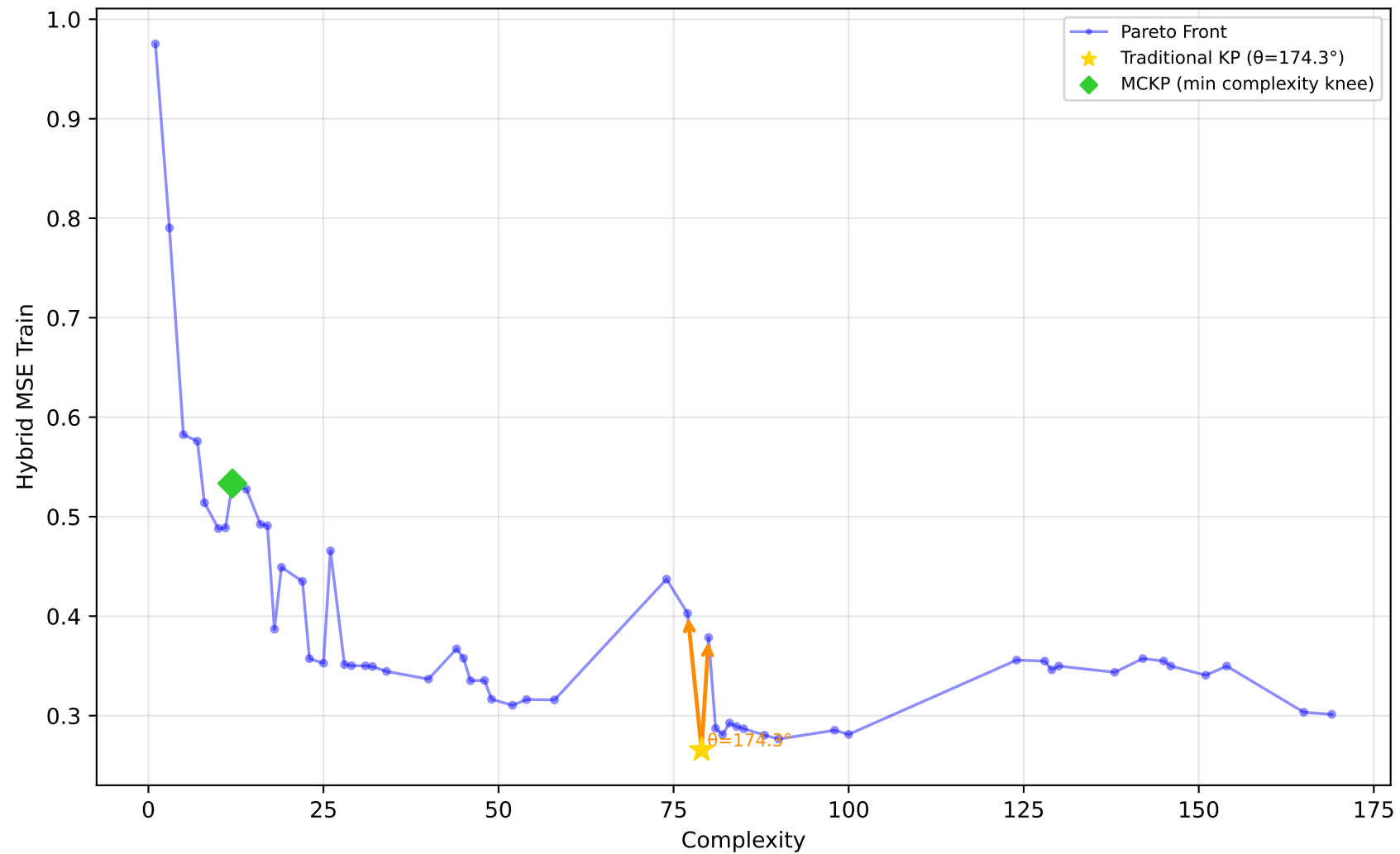
192_vineyard - Run 14 - SVP - Hybrid MSE Train \lambda_1=0.70, \bar{\lambda}_2=0.70, \lambda_3=0.90 | Difficulty: 0.72 | Method: hmr
