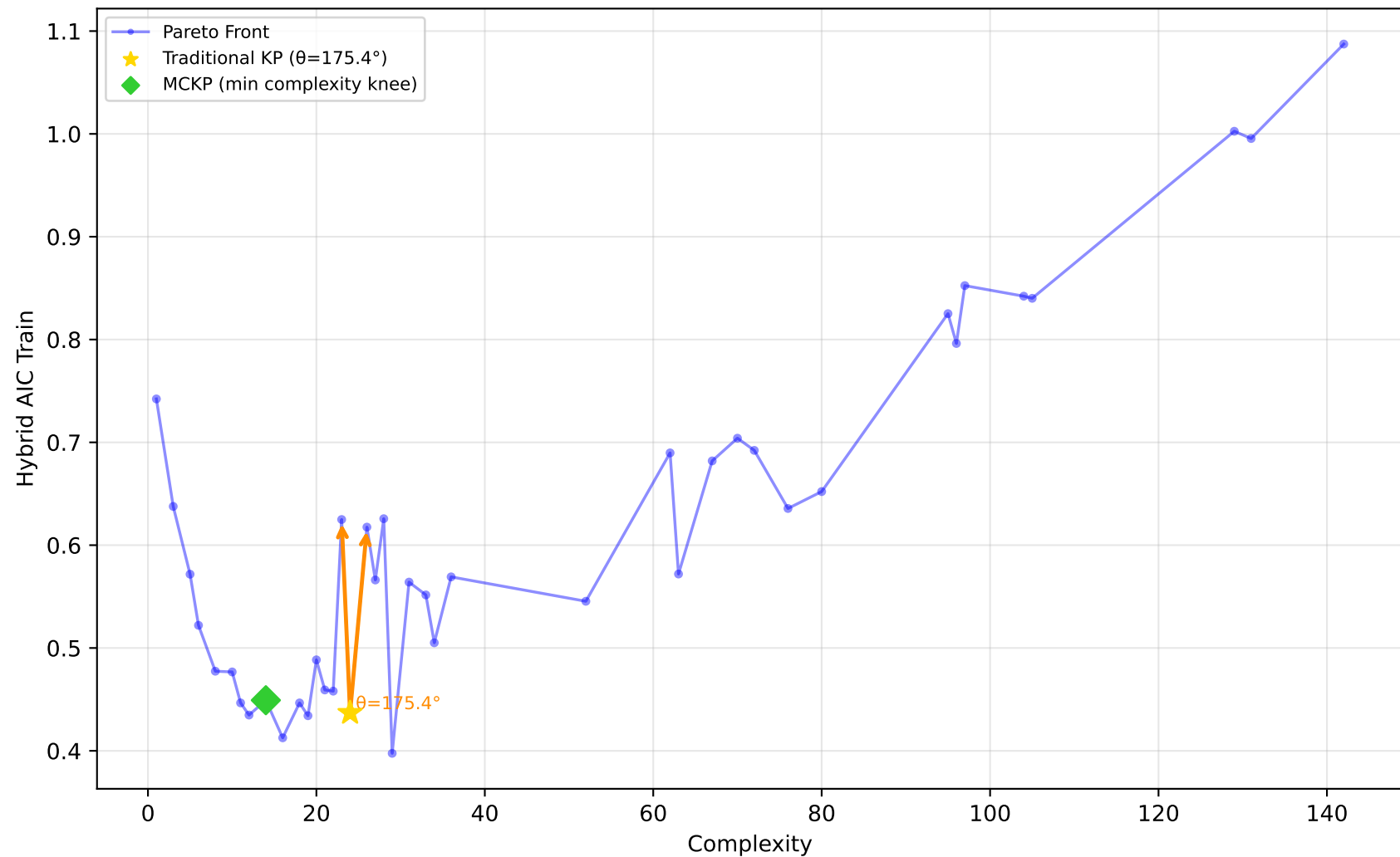
192_vineyard - Run 15 - MVP - Hybrid AIC Train \lambda_1=0.00, \bar{\lambda}_2=0.30, \lambda_3=1.00 | Difficulty: 1.00 | Method: hmr
