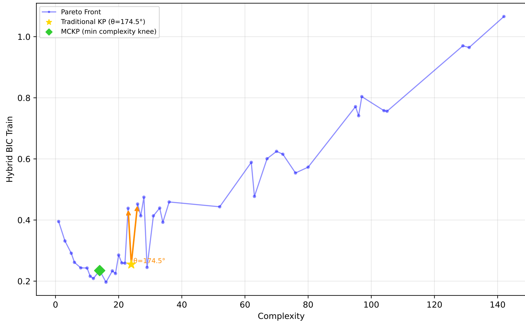
192_vineyard - Run 15 - MVP - Hybrid BIC Train \lambda_1=0.00, \bar{\lambda}_2=0.30, \lambda_3=1.00 | Difficulty: 1.00 | Method: hmr
