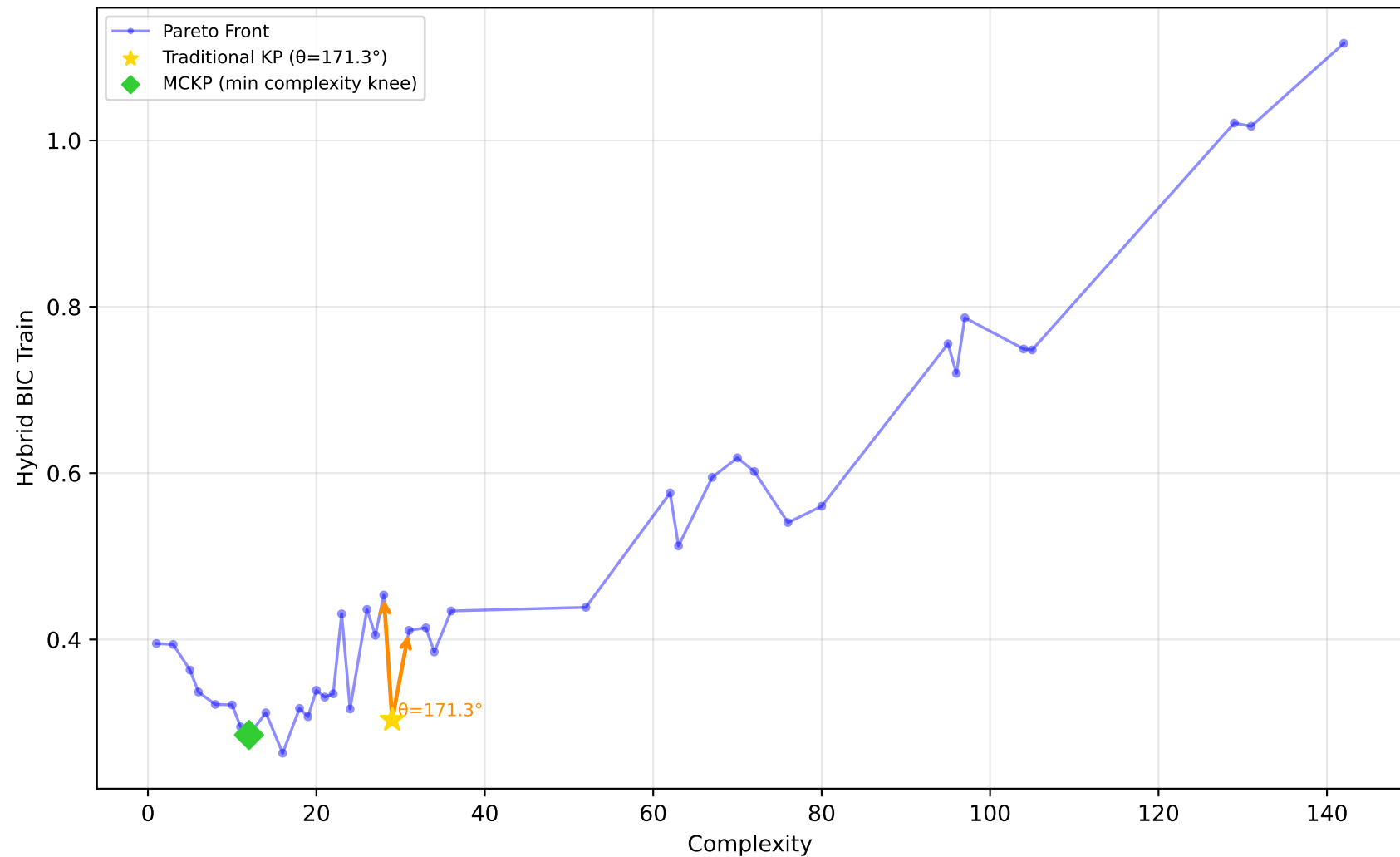
192_vineyard - Run 15 - MVP - Hybrid BIC Train \lambda_1=0.40, \bar{\lambda}_2=0.00, \lambda_3=1.00 | Difficulty: 1.00 | Method: hmr
