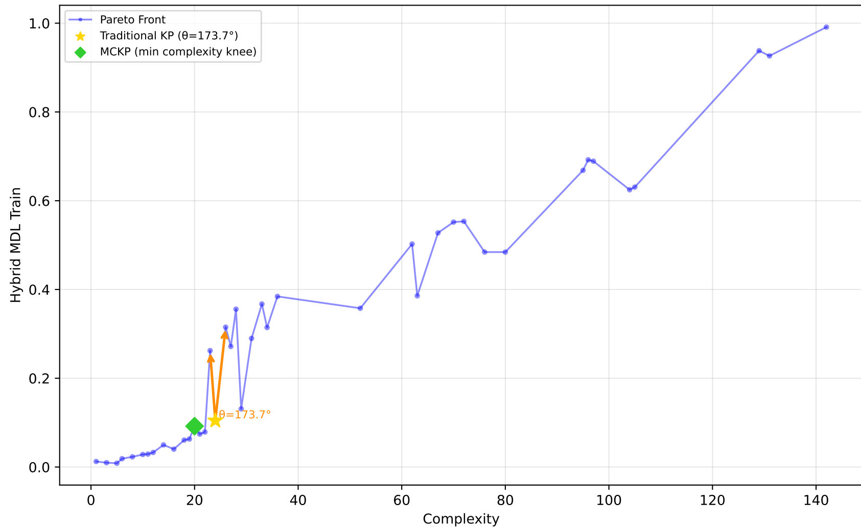
192_vineyard - Run 15 - MVP - Hybrid MDL Train \lambda_1=0.00, \lambda_2=0.30, \lambda_3=1.00 | Difficulty: 1.00 | Method: hmr
