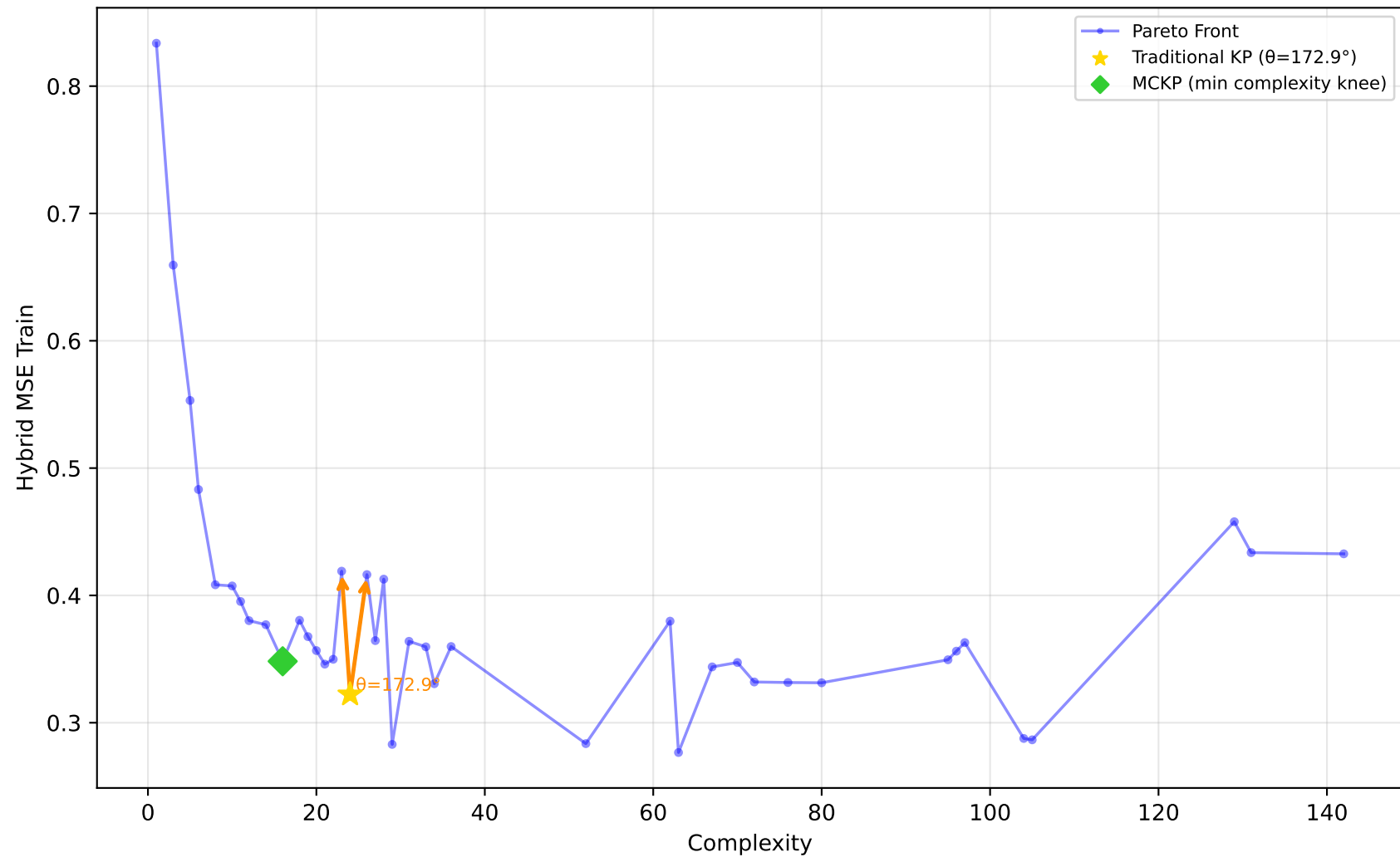
192_vineyard - Run 15 - MVP - Hybrid MSE Train \lambda_1=0.40, \lambda_2=0.00, \lambda_3=1.00 | Difficulty: 1.00 | Method: hmr
