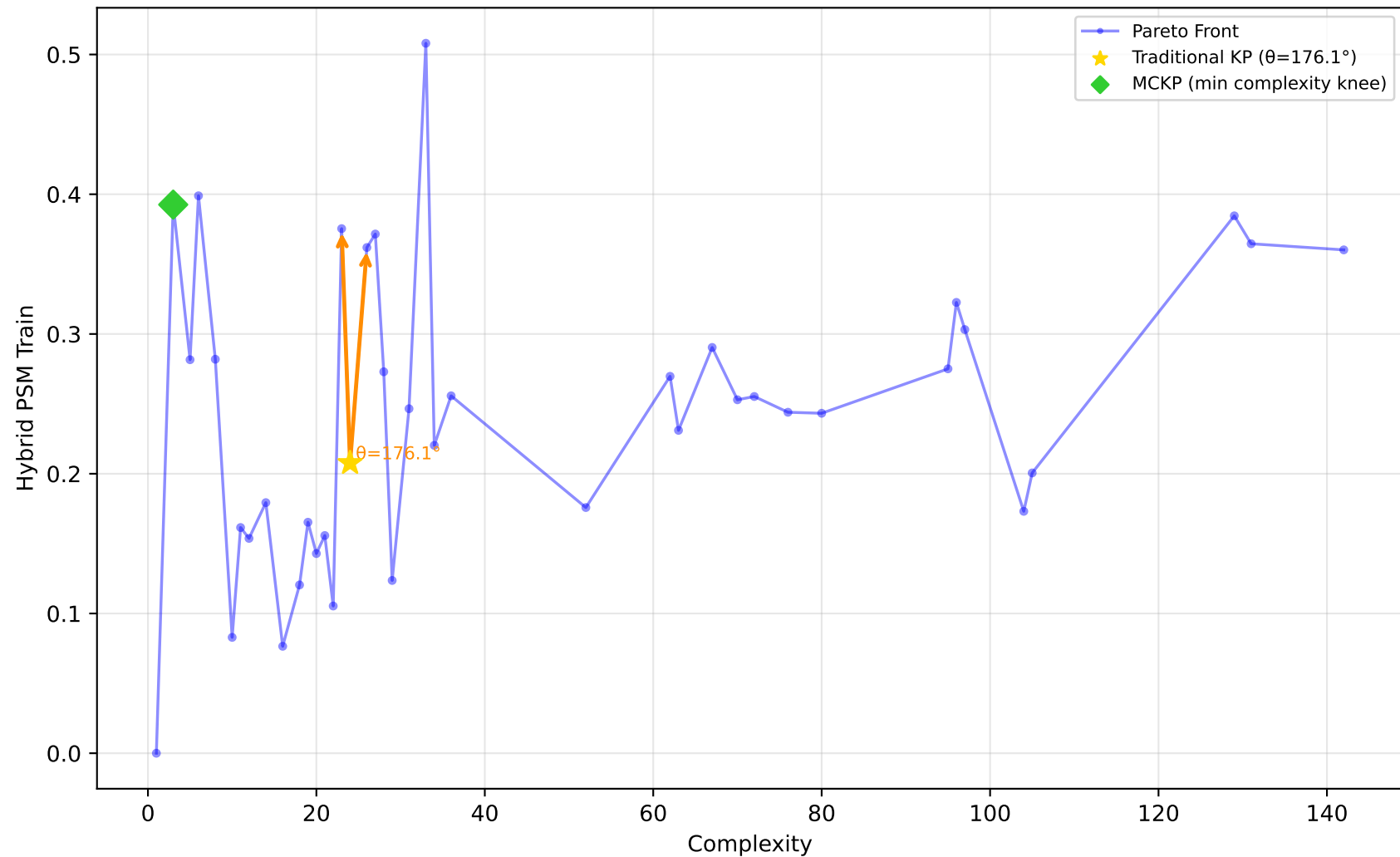
192_vineyard - Run 15 - MVP - Hybrid PSM Train \lambda_1=0.40, \lambda_2=0.00, \lambda_3=1.00 | Difficulty: 1.00 | Method: hmr
