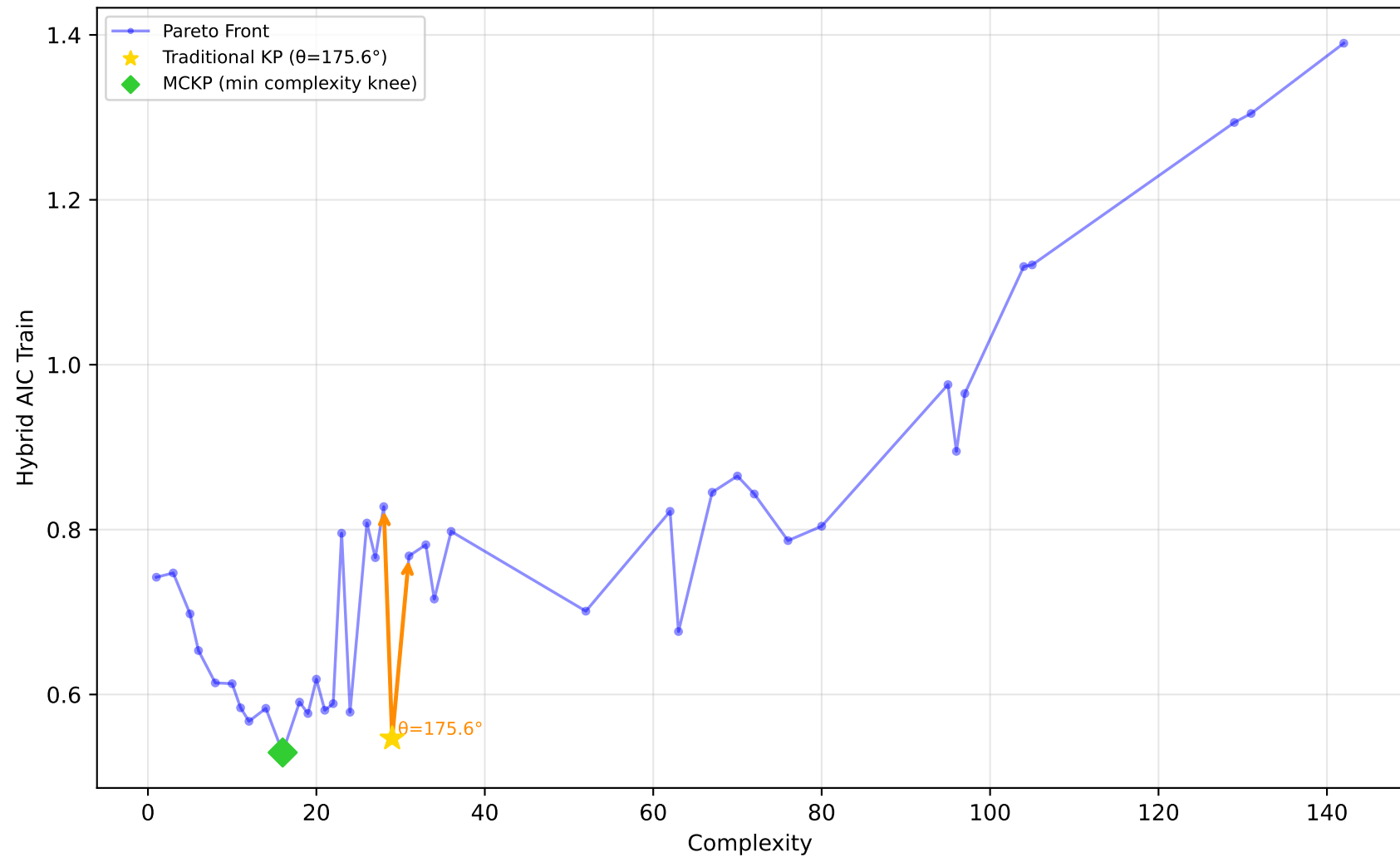
192_vineyard - Run 15 - SVP - Hybrid AIC Train \lambda_1=0.70, \bar{\lambda}_2=0.70, \lambda_3=0.90 | Difficulty: 1.00 | Method: hmr
