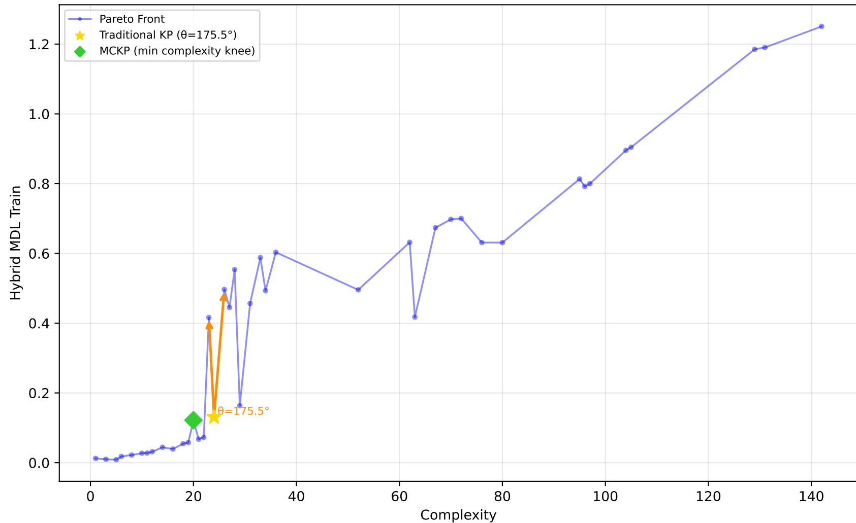
192_vineyard - Run 15 - SVP - Hybrid MDL Train \lambda_1=0.00, \lambda_2=1.00, \lambda_3=1.00 | Difficulty: 1.00 | Method: hmr
