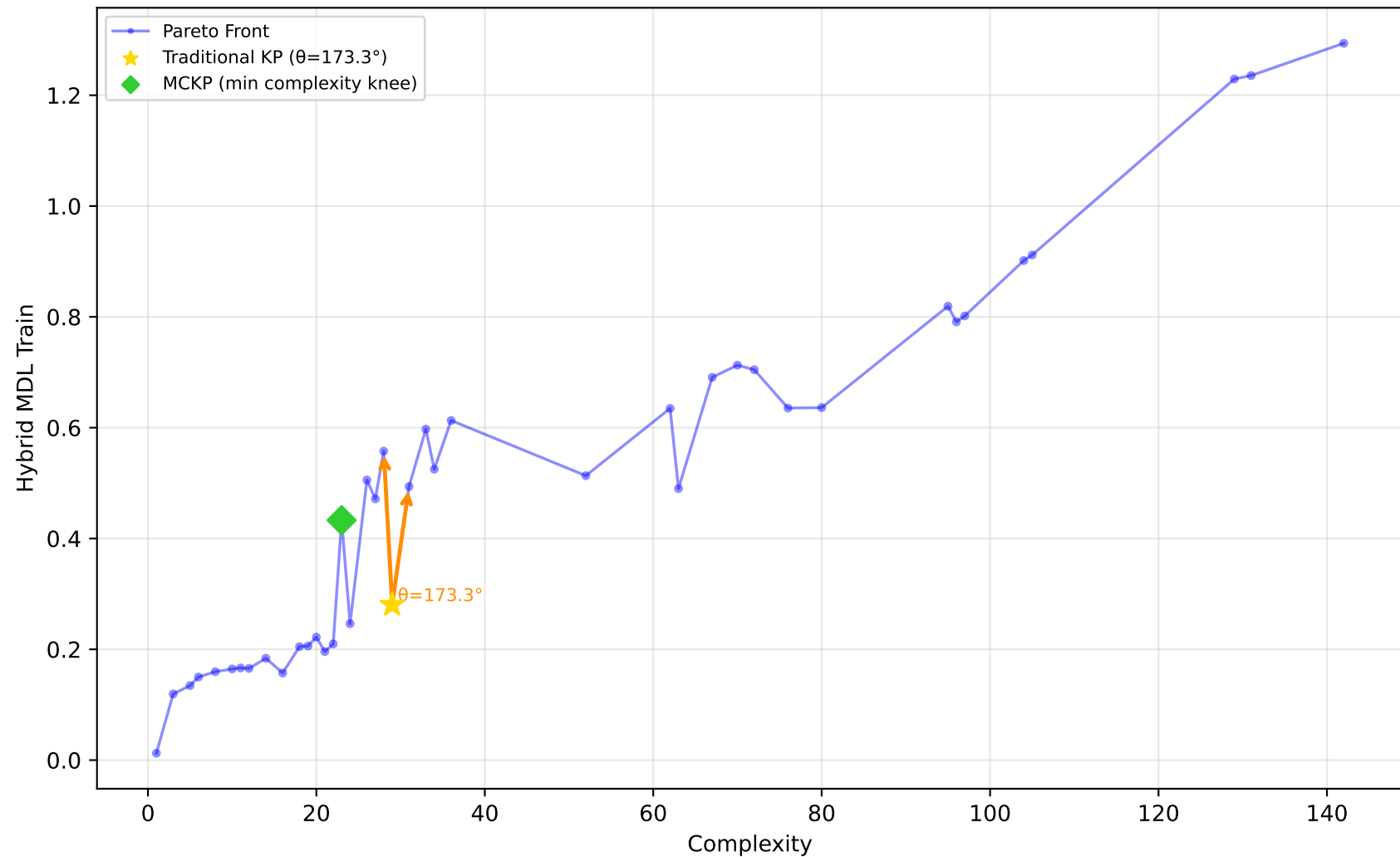
192_vineyard - Run 15 - SVP - Hybrid MDL Train \lambda_1=0.70, \bar{\lambda}_2=0.70, \lambda_3=0.90 | Difficulty: 1.00 | Method: hmr
