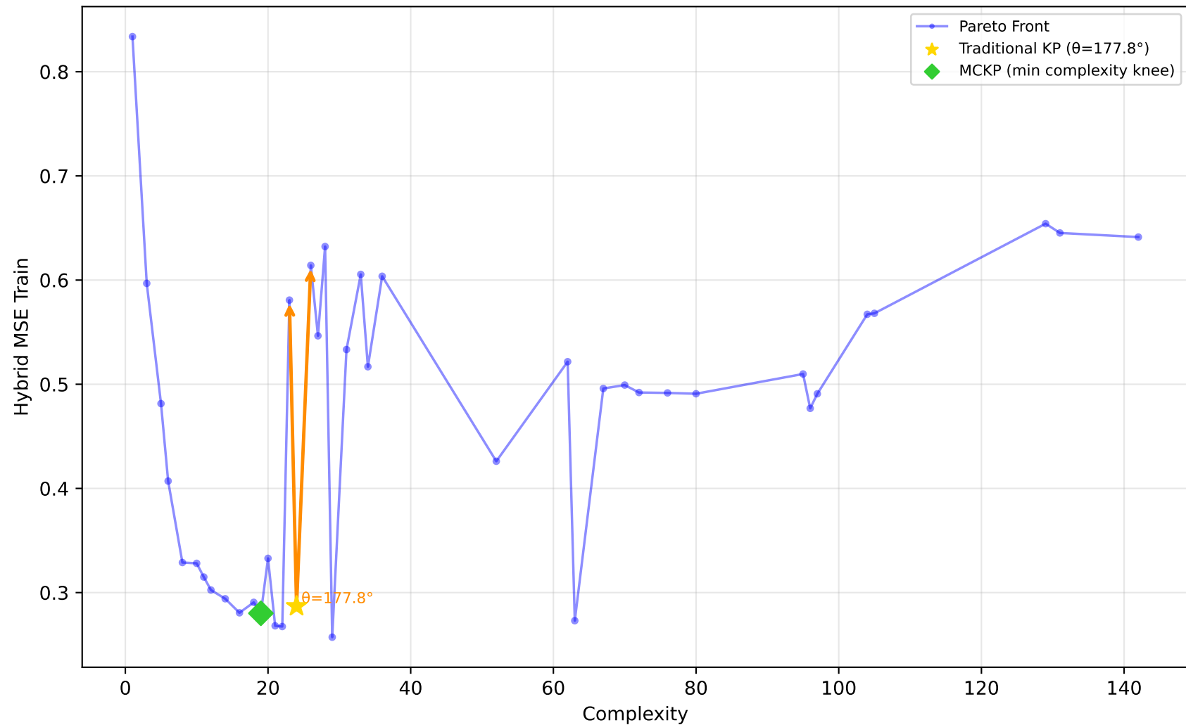
192_vineyard - Run 15 - SVP - Hybrid MSE Train \lambda_1=0.00, \bar{\lambda}_2=1.00, \lambda_3=1.00 | Difficulty: 1.00 | Method: hmr
