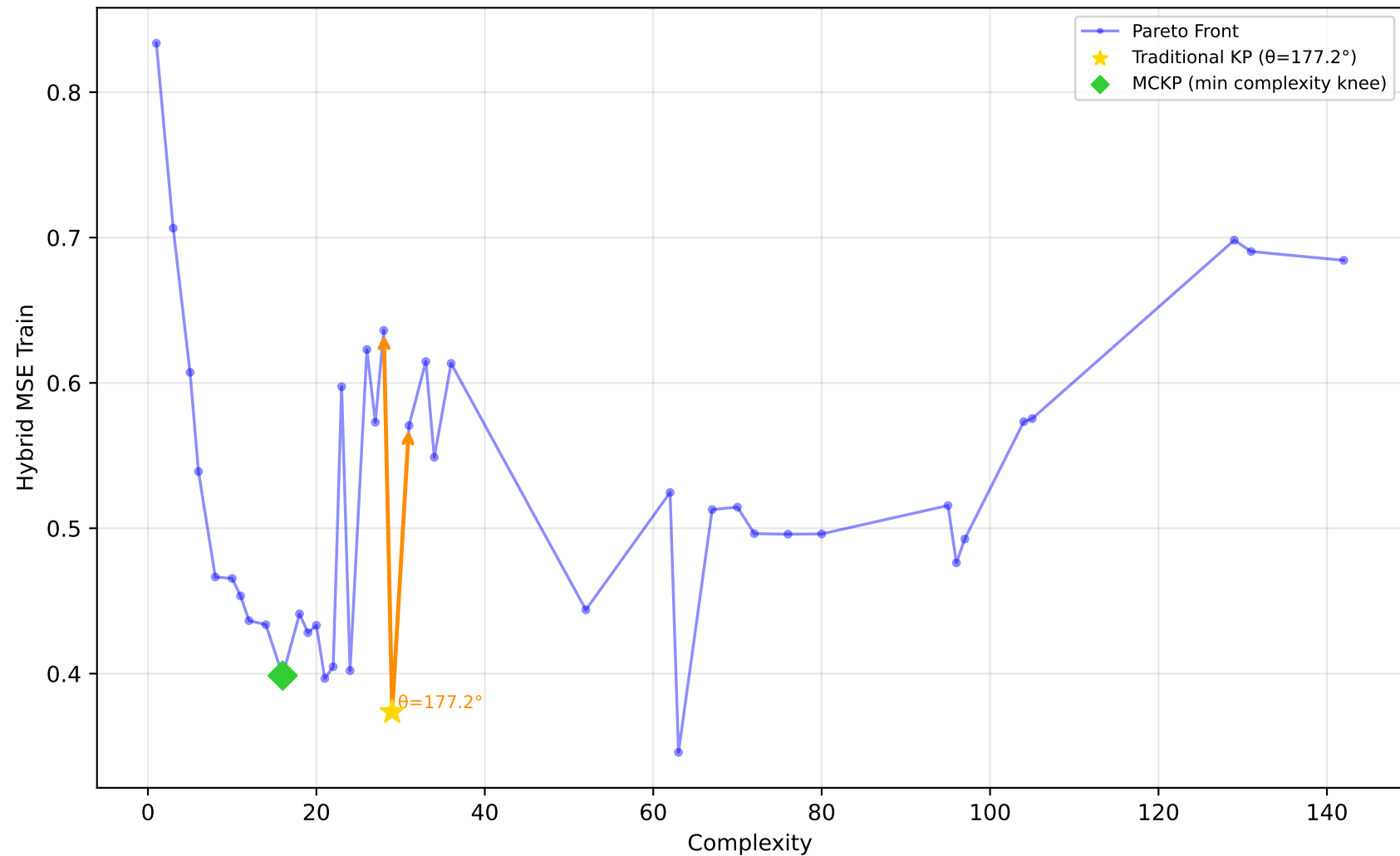
192_vineyard - Run 15 - SVP - Hybrid MSE Train \lambda_1=0.70, \lambda_2=0.70, \lambda_3=0.90 | Difficulty: 1.00 | Method: hmr
