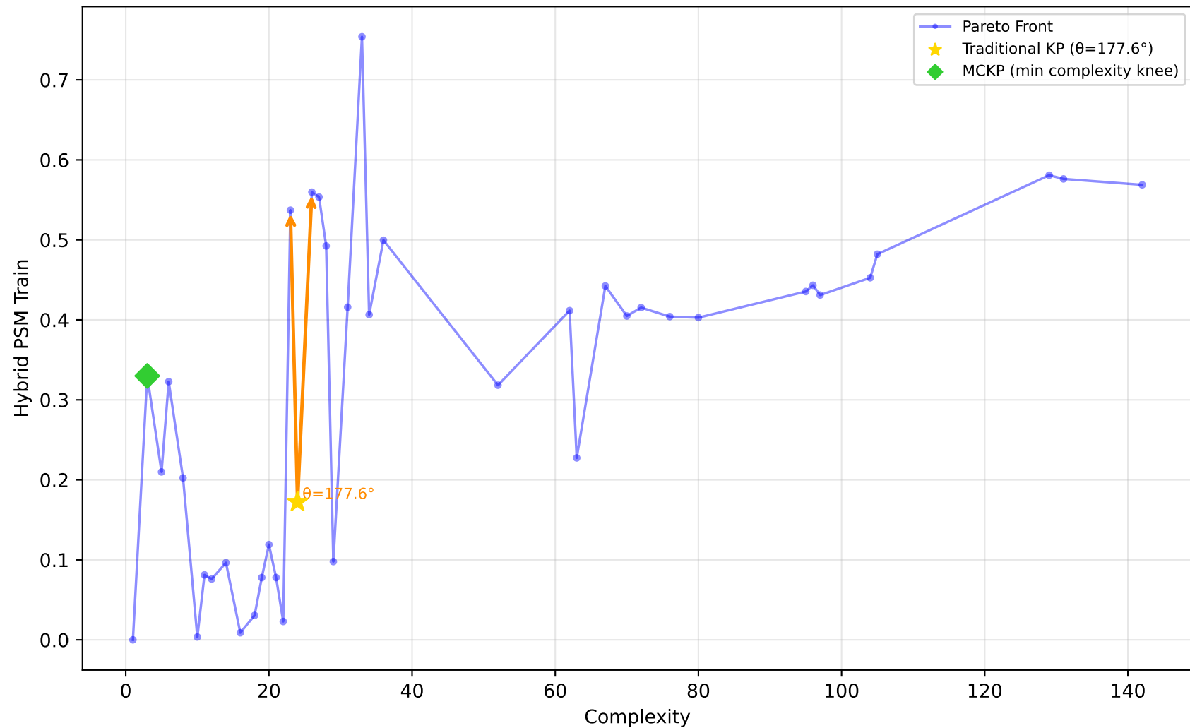
192_vineyard - Run 15 - SVP - Hybrid PSM Train \lambda_1=0.00, \bar{\lambda}_2=1.00, \lambda_3=1.00 | Difficulty: 1.00 | Method: hmr
