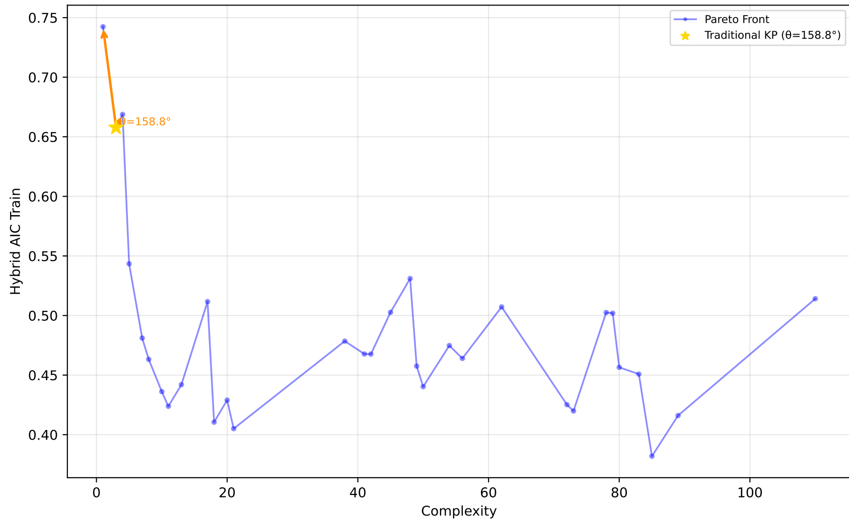
192_vineyard - Run 16 - MVP - Hybrid AIC Train \lambda_1=0.40, \bar{\lambda}_2=0.00, \lambda_3=1.00 | Difficulty: 1.00 | Method: hmr
