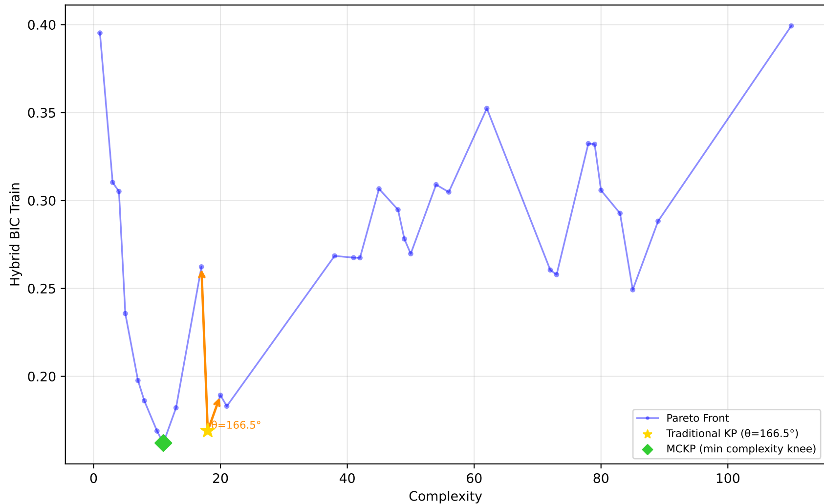
192_vineyard - Run 16 - MVP - Hybrid BIC Train \lambda_1=0.00 , \bar{\lambda}_2=0.30 , \lambda_3=1.00 | Difficulty: 1.00 | Method: hmr
