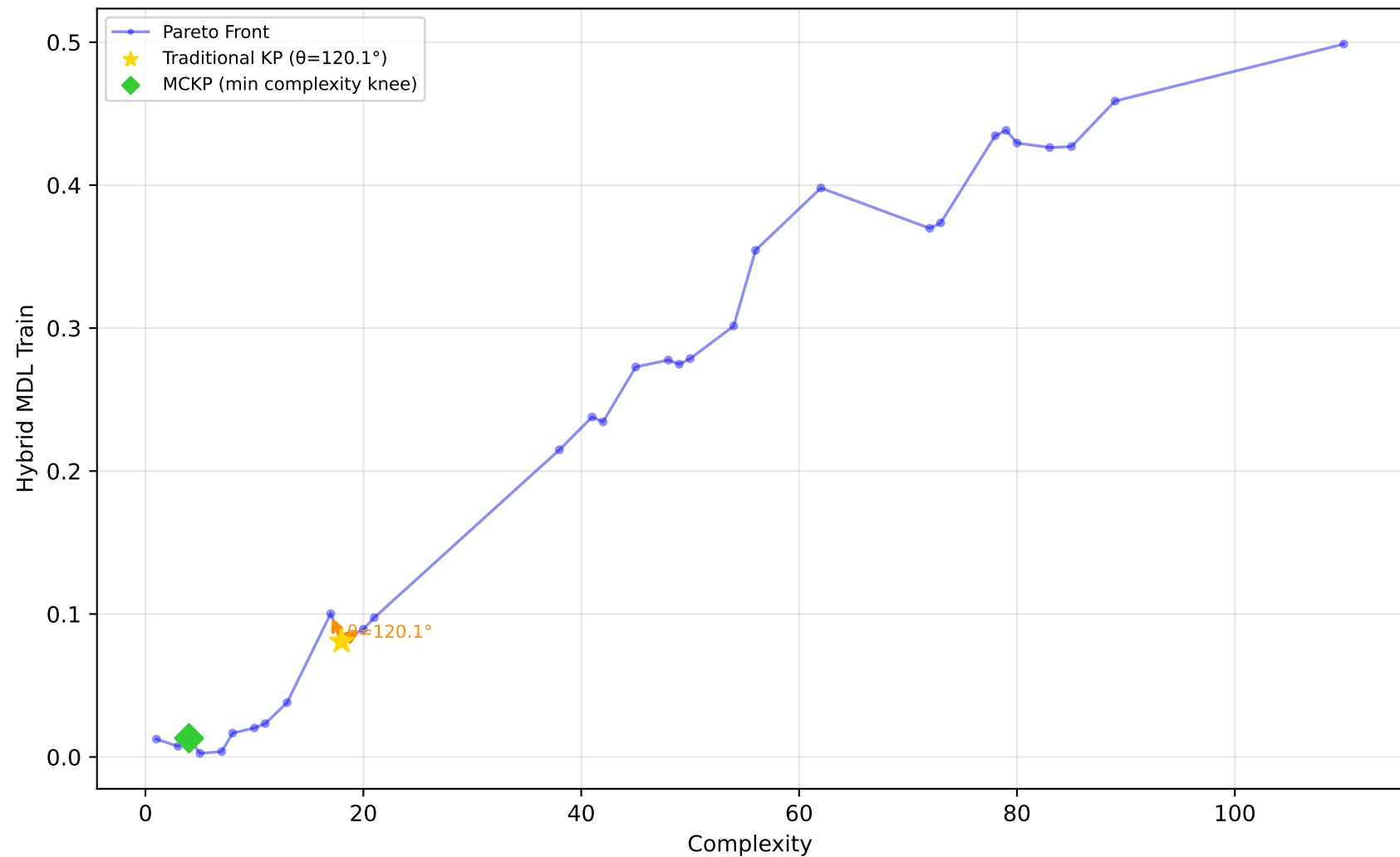
192_vineyard - Run 16 - MVP - Hybrid MDL Train \lambda_1=0.00, \lambda_2=0.30, \lambda_3=1.00 | Difficulty: 1.00 | Method: hmr
