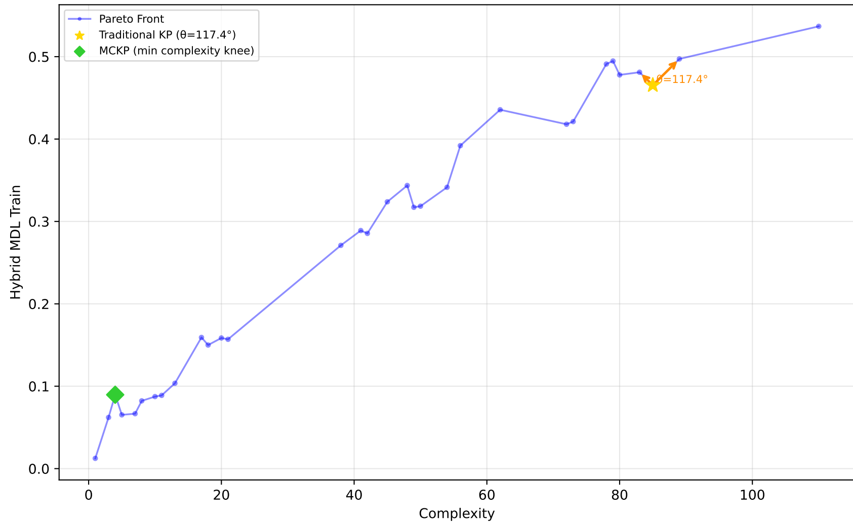
192_vineyard - Run 16 - MVP - Hybrid MDL Train \lambda_1=0.40, \bar{\lambda}_2=0.00, \lambda_3=1.00 | Difficulty: 1.00 | Method: hmr
