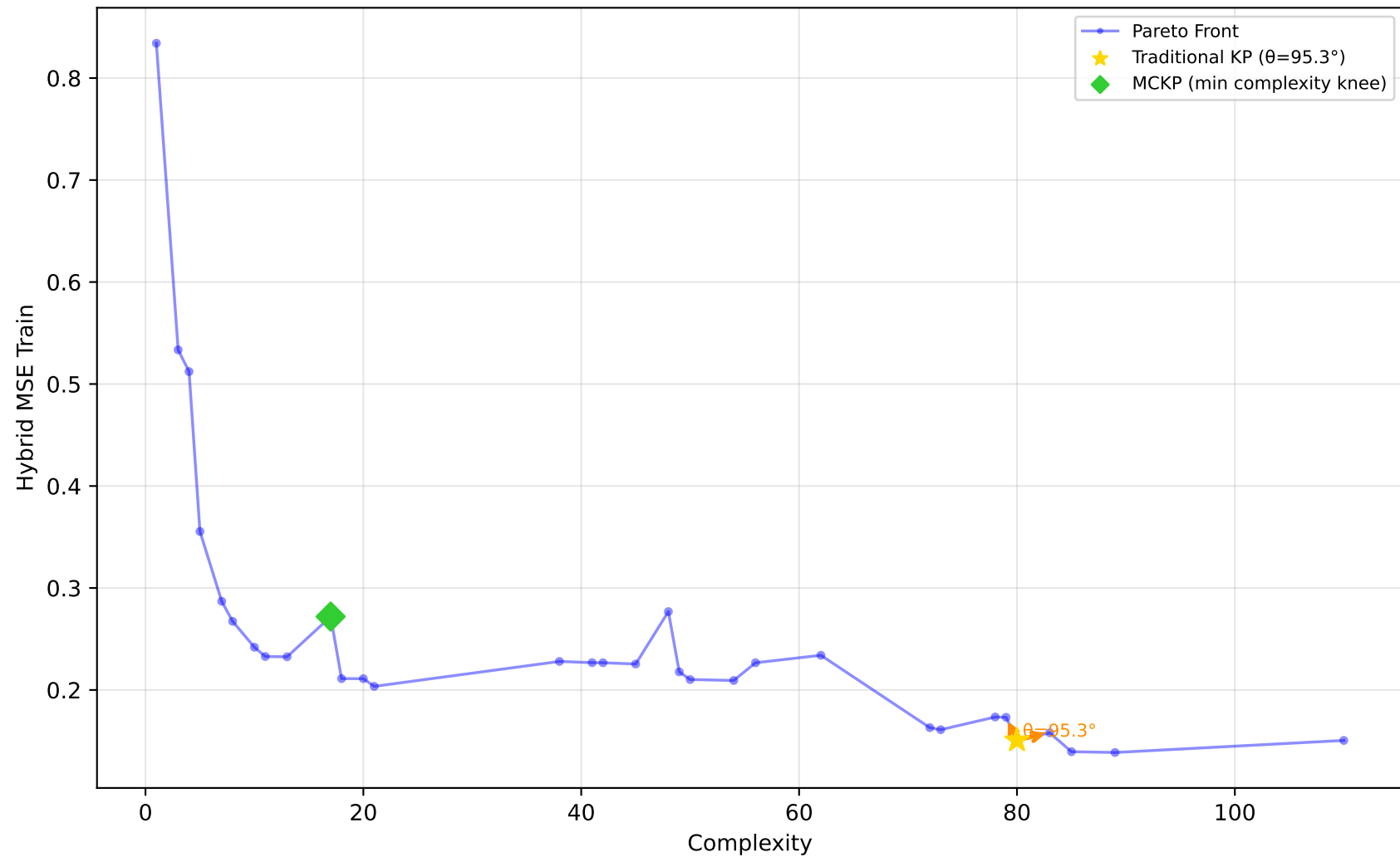
192_vineyard - Run 16 - MVP - Hybrid MSE Train \lambda_1=0.00, \lambda_2=0.30, \lambda_3=1.00 | Difficulty: 1.00 | Method: hmr
