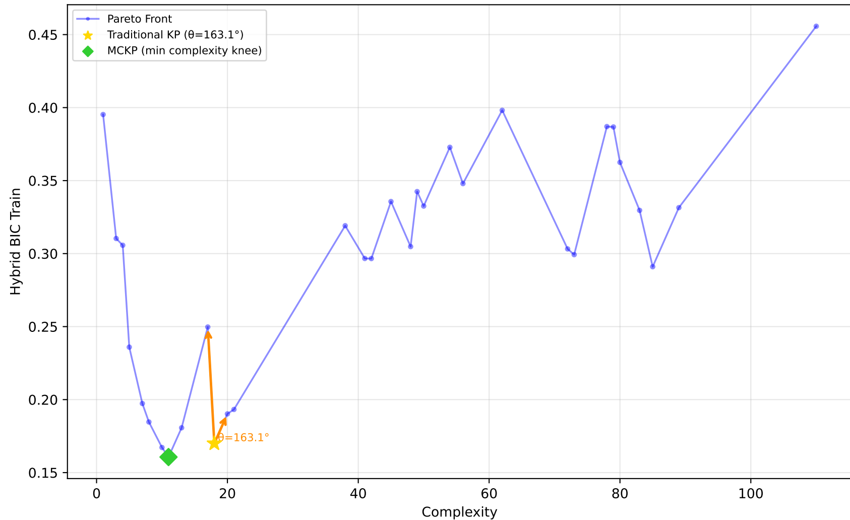
192_vineyard - Run 16 - SVP - Hybrid BIC Train \lambda_1=0.00, \bar{\lambda}_2=1.00, \lambda_3=1.00 | Difficulty: 1.00 | Method: hmr
