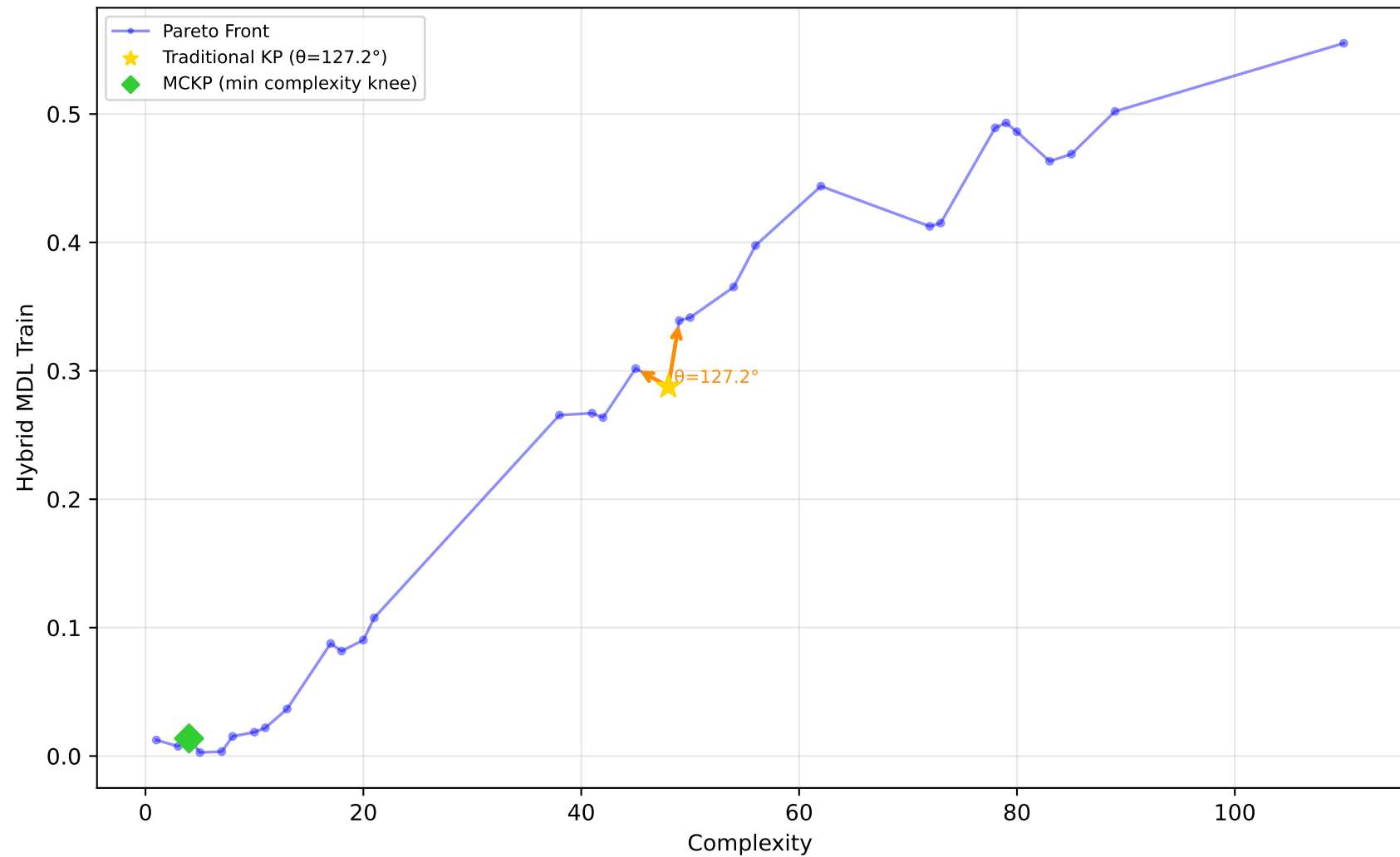
192_vineyard - Run 16 - SVP - Hybrid MDL Train \lambda_1=0.00, \lambda_2=1.00, \lambda_3=1.00 | Difficulty: 1.00 | Method: hmr
