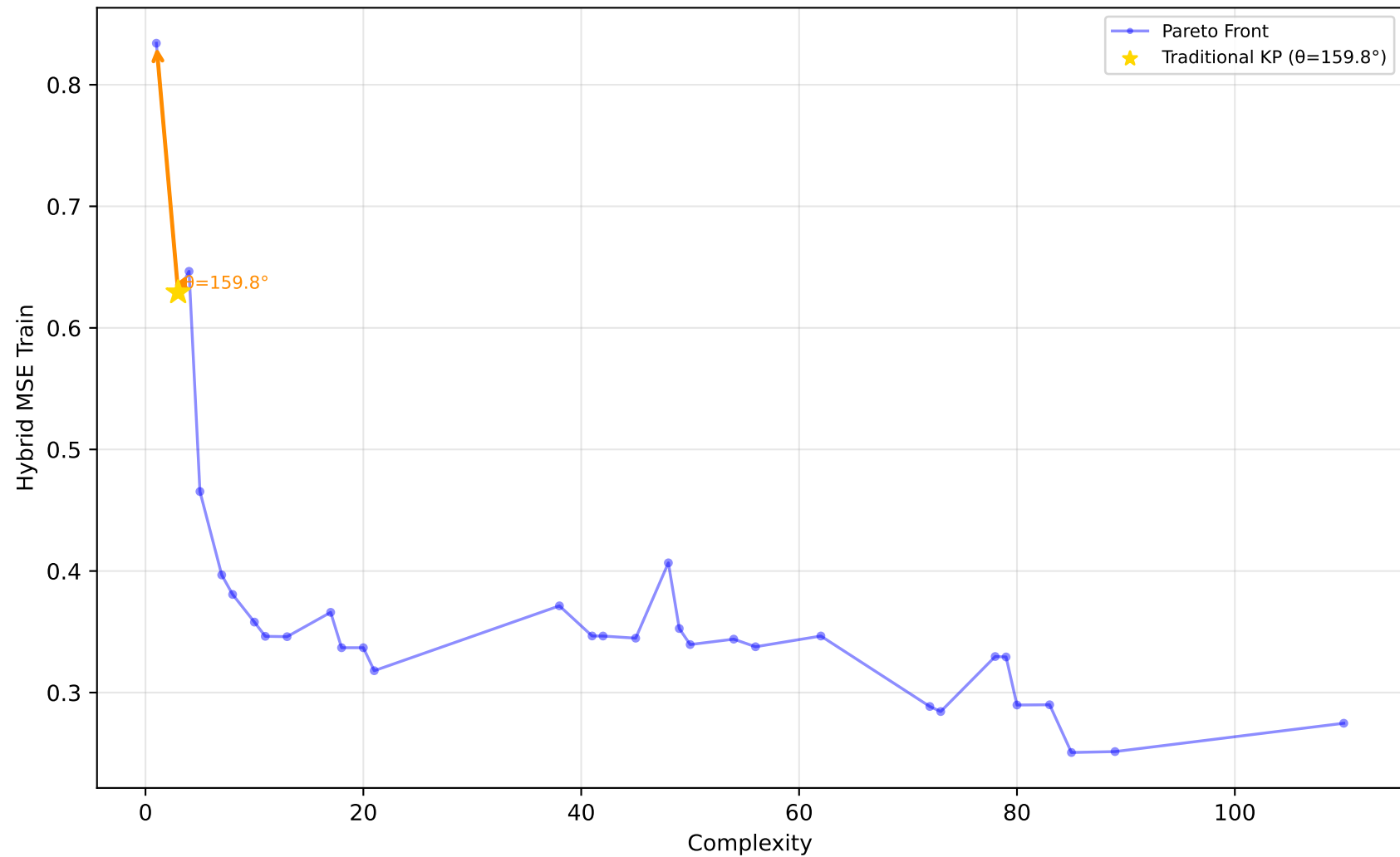
192_vineyard - Run 16 - SVP - Hybrid MSE Train \lambda_1=0.70, \bar{\lambda}_2=0.70, \lambda_3=0.90 | Difficulty: 1.00 | Method: hmr
