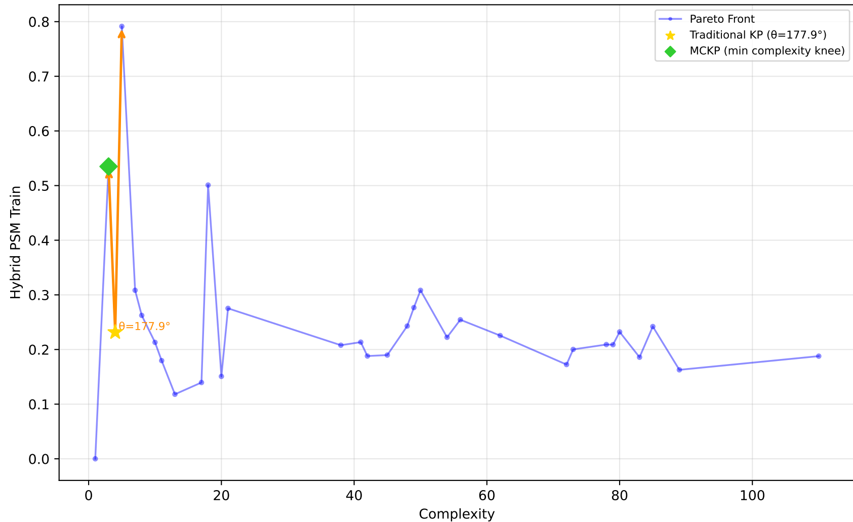
192_vineyard - Run 16 - SVP - Hybrid PSM Train \lambda_1=0.70, \bar{\lambda}_2=0.70, \lambda_3=0.90 | Difficulty: 1.00 | Method: hmr
