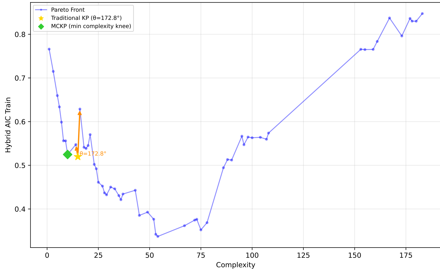
192_vineyard - Run 17 - MVP - Hybrid AIC Train \lambda_1=0.40, \bar{\lambda}_2=0.00, \lambda_3=1.00 | Difficulty: 0.71 | Method: hmr
